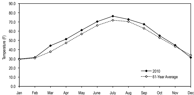
Figure 1-5. BNL 2010 Monthly Mean Temperature versus 61-Year Monthly Average.
