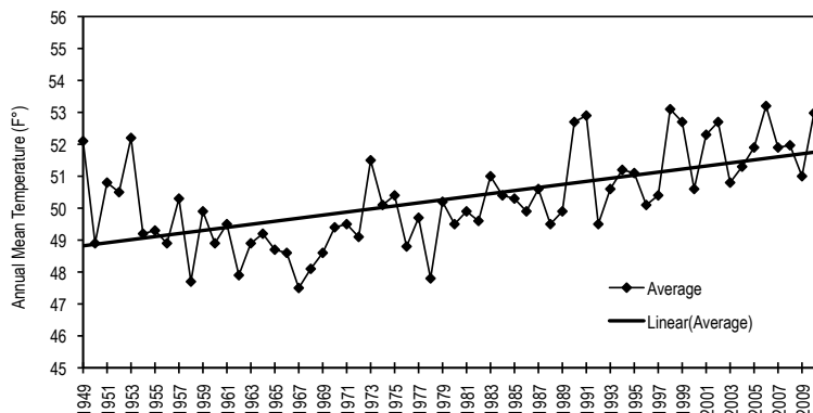
Figure 1-6. BNL 2010 Annual Mean Temperature Trend (61 Years).
