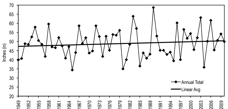
Figure 1-8. BNL 2010 Annual Precipitation Trend (61 Years).
