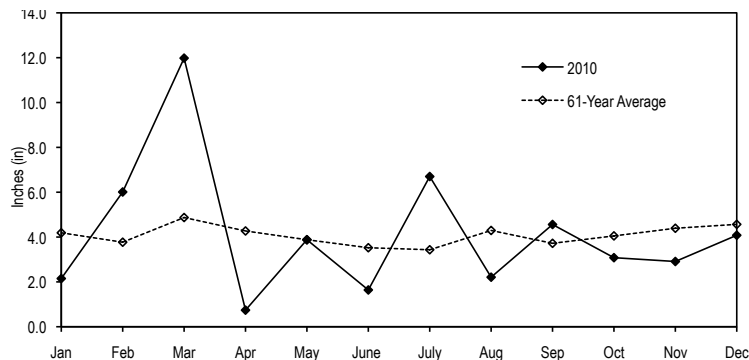
Figure 1-7. BNL 2010 Monthly Precipitation versus 61-Year Monthly Average.
