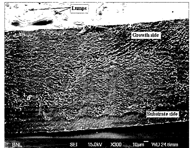
Figure 3: SEM picture of the cross-section of the sample 1 diamond.
