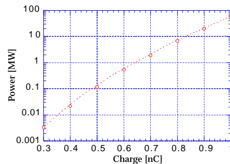
Figure 1: FEL radiation power dependence on charge
