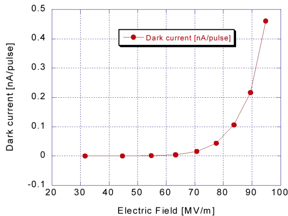
Fig. 2 Dark current measured under the rf conditioning with the 6 MW of rf power
