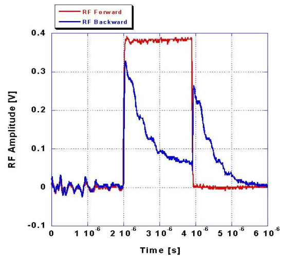
Fig.4 The rf forward and backward signal for the rf-gun cavity
