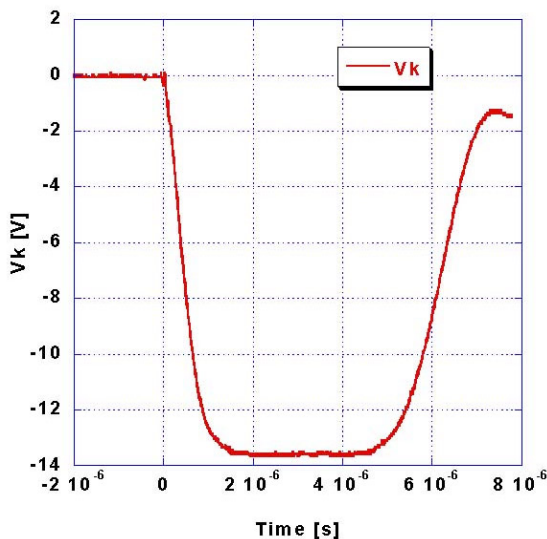
Fig. 3 Typical output of klystron voltage at the operation point of 140 kV
