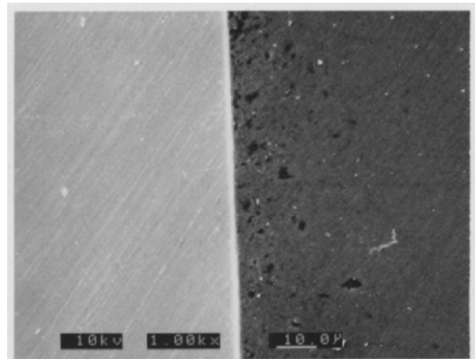
Fig. 1 Photograph of cathode surface around the contact area of Cu-Mg after the polishing
