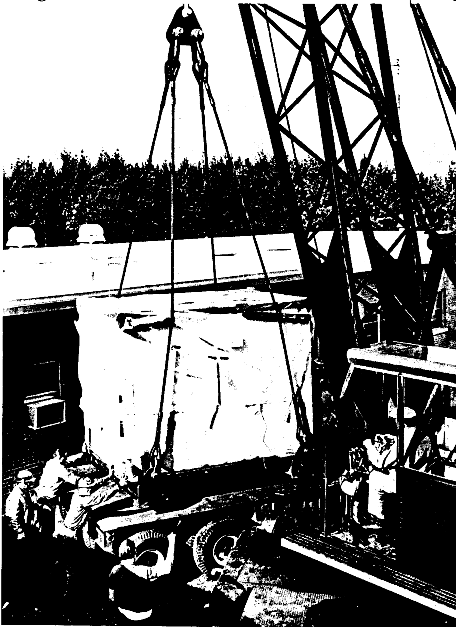
Shielded steel room being lifted by BNL's 80-ton crane in front of Medical Research Center.
