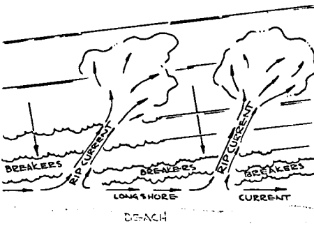
Schematic of nearshore circulation system with arrows indicating direction of water transport.
