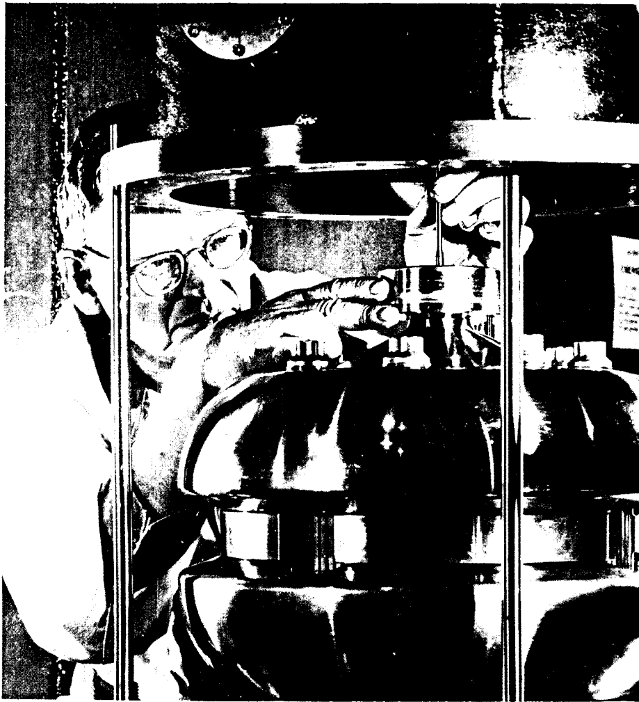
Fred Paffrath, Physics, is checking the condition of the shaft of the rotor of the Fast Neutron Chopper at the HFBR. The slender piece of steel, only 3/16-in. diameter supports the 650 pound rotor beneath it that spins at 10,000 rpm. This machine was first used in neutron physics experiments on June 7, 1966. It has run continuously since then with only occasional shutdowns for routine maintenance. —Rosen
