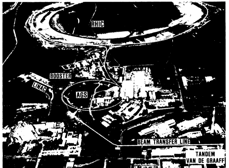
The accelerator chain for the proposed Relativistic Heavy Ion Collider (RHIC): After heavy ions are generated in the Tandem, they will travel to the Booster, then to the AGS, and ultimately to RHIC.
