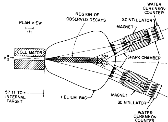
A diagram of the experimental setup for AGS experiment E181.
