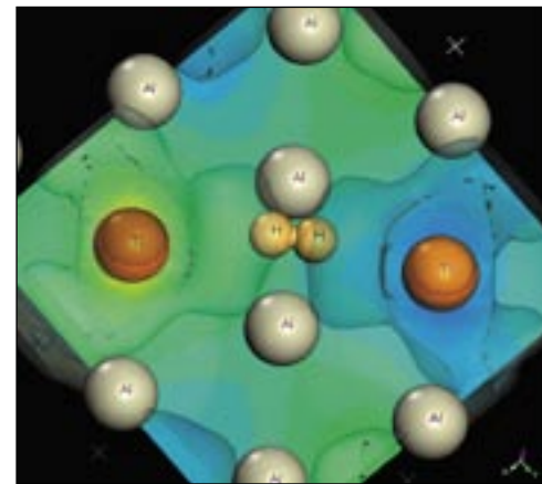
The arrangement of titanium (Ti) atoms on or near the aluminum (Al) surface determines the way molecular hydrogen (H 2 ) is chemically absorbed. The picture shows a top-view of the surface in the initial stages of hydrogen adduct formation on one of the possible titanium-aluminum arrangements.
