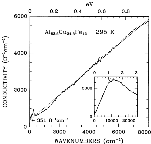
FIG. 2. The optical conductivity of the quasicrystal \text{Al}_{63.5}\text{Cu}_{24.5}\text{Fe}_{12} at 295 \text{ K} from 40 to 8000 \text{ cm}^{-1} obtained by Kramers-Kronig analysis of the reflectance. The conductivity rises linearly from the low dc value to a magnitude of 6000 \Omega^{-1} \text{ cm}^{-1} , a value typical for many metals in the visible. The dashed line is a least-squares fit to the data from 40 to 7500 \text{ cm}^{-1} . Inset: The behavior of the conductivity over a larger frequency range.
