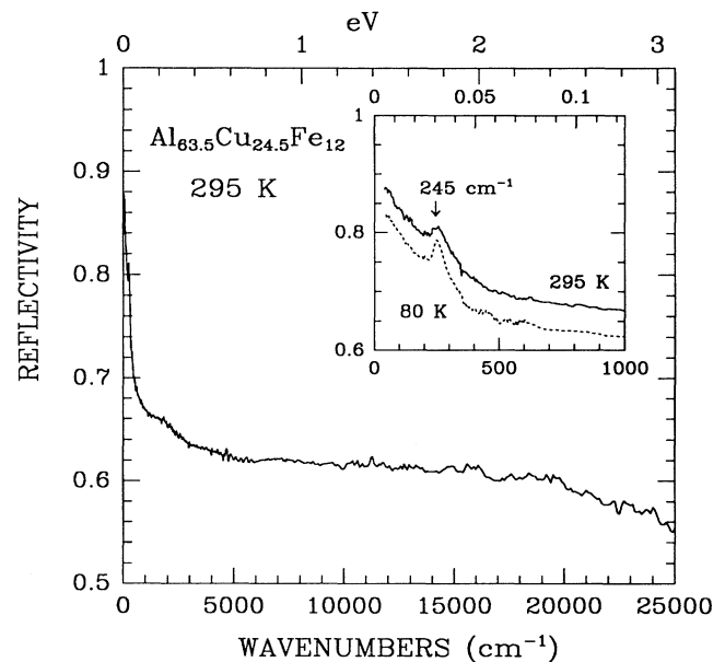
FIG. 1. The reflectivity of \text{Al}_{63.5}\text{Cu}_{24.5}\text{Fe}_{12} at 295 K from 40 to 25000\text{ cm}^{-1} . Inset: The reflectance at 295 K (solid line) and at 80 K (dashed line) on an expanded scale. The shoulder at \approx 250\text{ cm}^{-1} is clearly visible.
