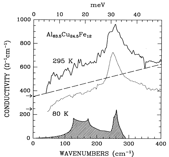
FIG. 3. The low-frequency optical conductivity of \text{Al}_{63.5}\text{Cu}_{24.5}\text{Fe}_{12} at 295 \text{ K} (solid line) and at 80 \text{ K} (dotted line). The straight dashed line is the result of the least-squares fit to the room-temperature data shown in Fig. 2. The arrows indicate the measured dc conductivity at 295 \text{ K} (top) and 80 \text{ K} (bottom). The shaded area at the bottom of the figure is the phonon density of states in Al (with the frequency and amplitude adjusted for the different reduced mass in the formula). We believe the structure at 250 \text{ cm}^{-1} and below is due to phonons activated by the quasicrystalline order.
