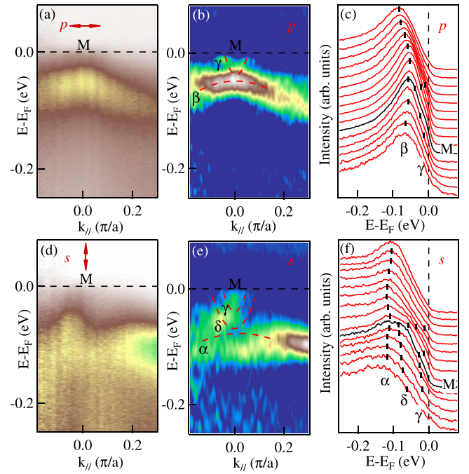
FIG. 3. The ARPES data around M along \Gamma\bar{M} direction with the linearly polarized light and photon energy h\nu = 36 eV at T = 20 K. (a) Intensity plot taken at M point in p geometry. (b) Second derivative [\partial^2 I(\omega, k)/\partial \omega^2] intensity plot of data in panel (a) to illustrate band dispersion. (c) EDCs of the data in panel (a). The markers are band dispersions plotted as guide to the eye. (d)-(f) The same as panels (a), (b), and (c), respectively, but taken in s geometry. The electric fields are indicated by arrows in (a) and (d).
