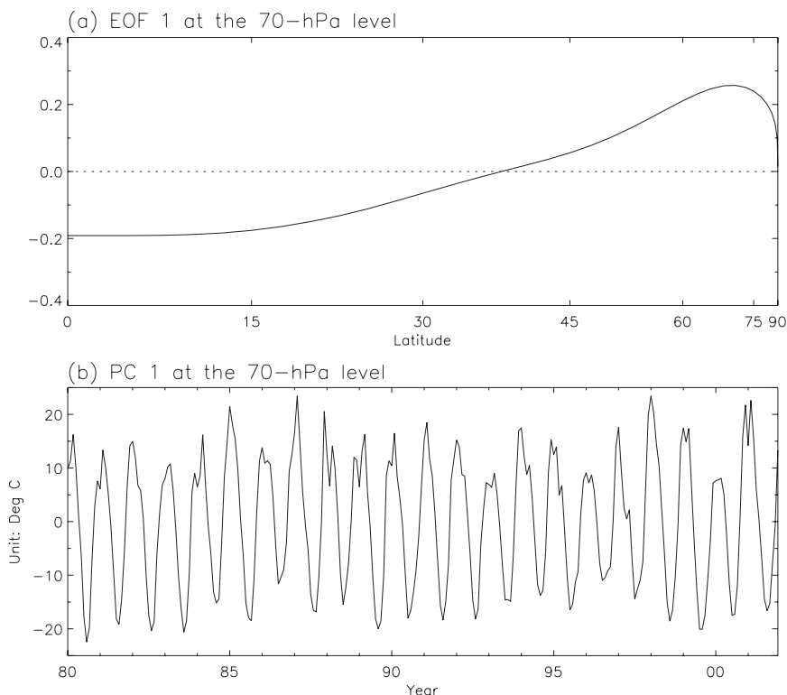
FIG. 2. As in Fig. 1, but for T^* at the 70-hPa level from 1980 to 2001.
