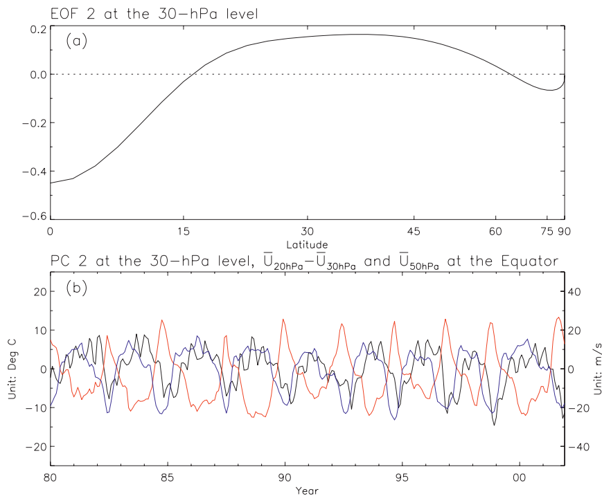
FIG. 5. (a) The second leading EOF of T^* at the 30-hPa level from 1980 to 2001. The horizontal scale is as in Fig. 1a. (b) The corresponding second principal component time series of the zonal mean equatorial zonal wind at the 30-hPa level represented by \bar{u}_{20\text{hPa}} - \bar{u}_{30\text{hPa}} (red line), and the zonal mean equatorial zonal wind at the 50-hPa level (blue line).
