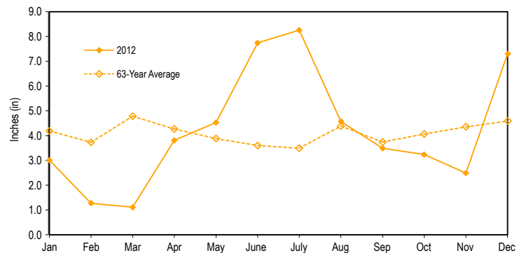
Figure 1-7. BNL 2012 Monthly Precipitation versus 63-Year Monthly Average.
