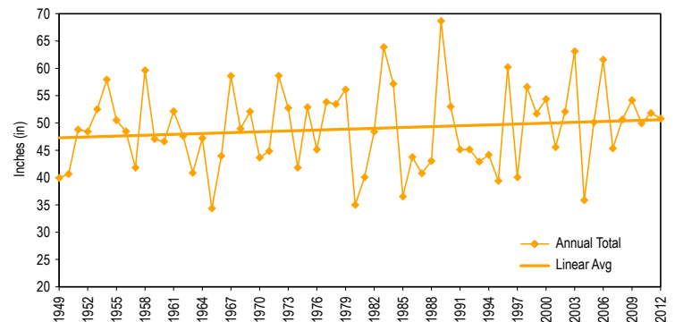
Figure 1-8. BNL 2012 Annual Precipitation Trend (63 Years).
