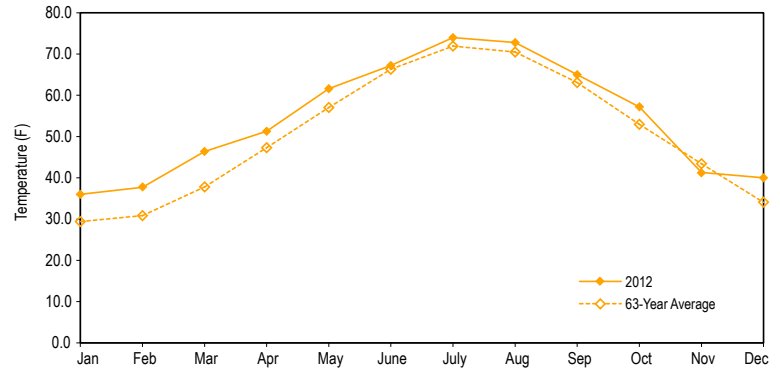
Figure 1-5. BNL 2012 Monthly Mean Temperature versus 63-Year Monthly Average.
