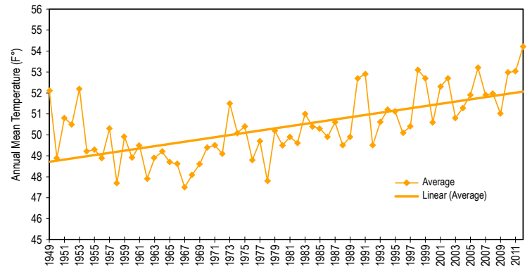
Figure 1-6. BNL 2012 Annual Mean Temperature Trend (63 Years).
