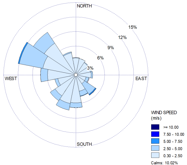
Wind Rose for Jan 1 to Dec 31, 2024 taken at the 10m height.
