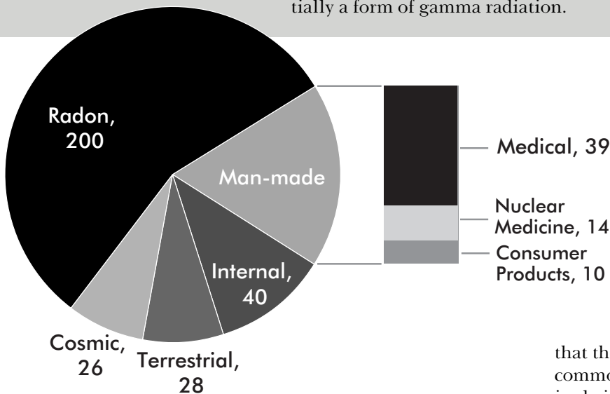
Figure 4-1. Typical Annual Radiation Doses from Natural and Man-Made Sources (mrem) Source: NCRP Report No. 93.
