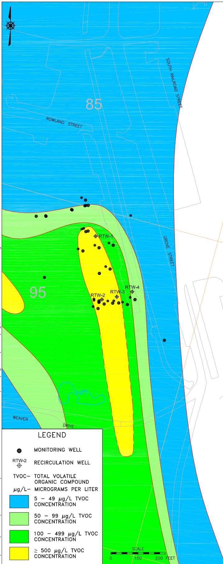
2000 TVOC PLUME DISTRIBUTION
