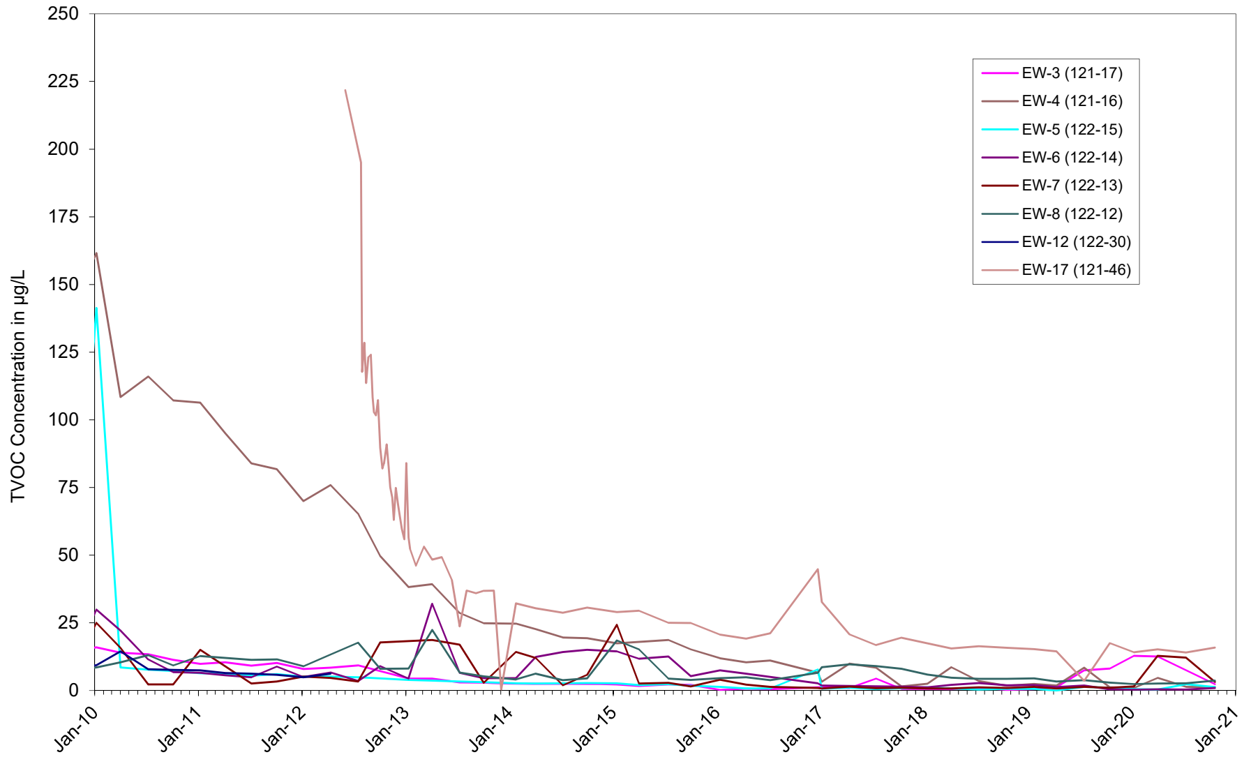
Figure 3.2.3-4 OU III South Boundary Groundwater Remediation System Total Volatile Organic Compounds in Extraction Wells 2010 through 2020
