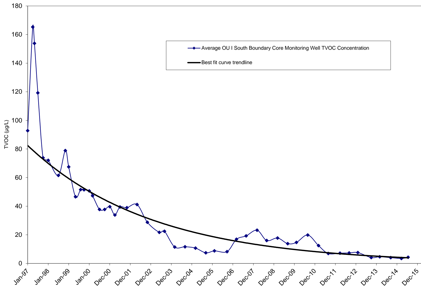
Figure 3.1-10 OU I South Boundary Groundwater Remediation System Average Core Monitoring Well TVOC Concentration
