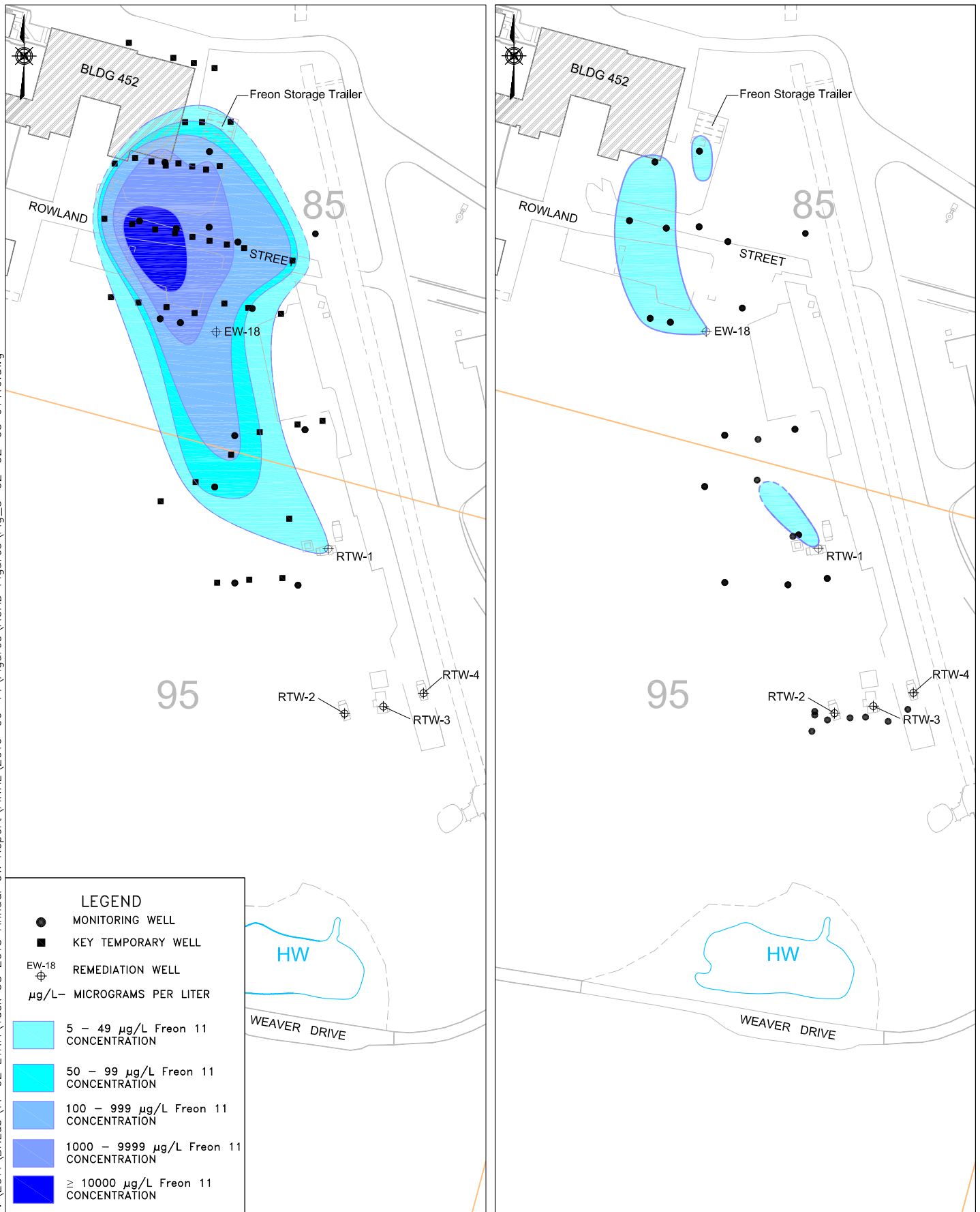
2011 FREON-11 PLUME DISTRIBUTION
