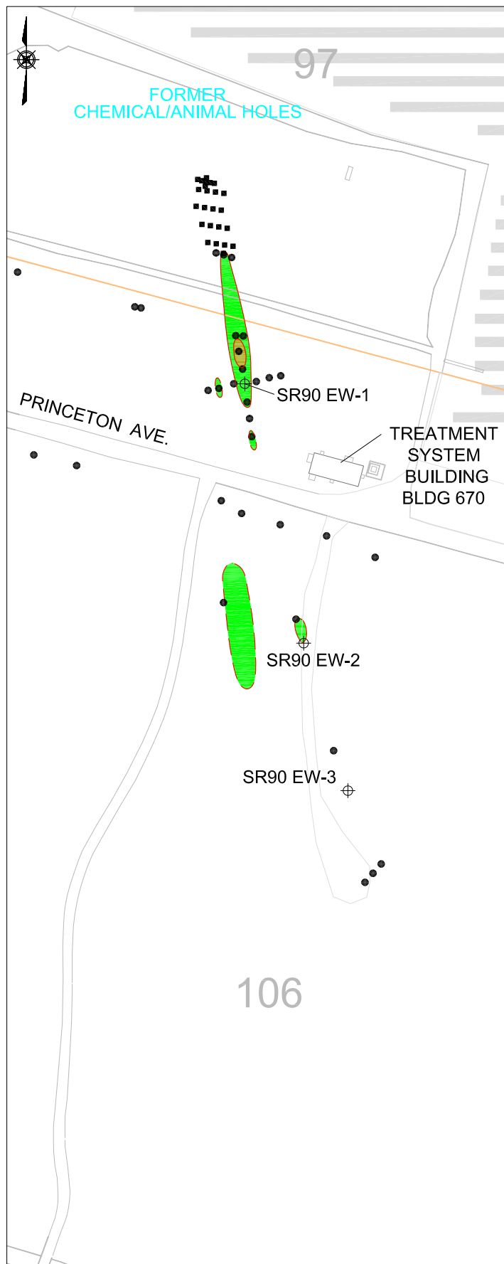
2015 Sr-90 PLUME DISTRIBUTION
