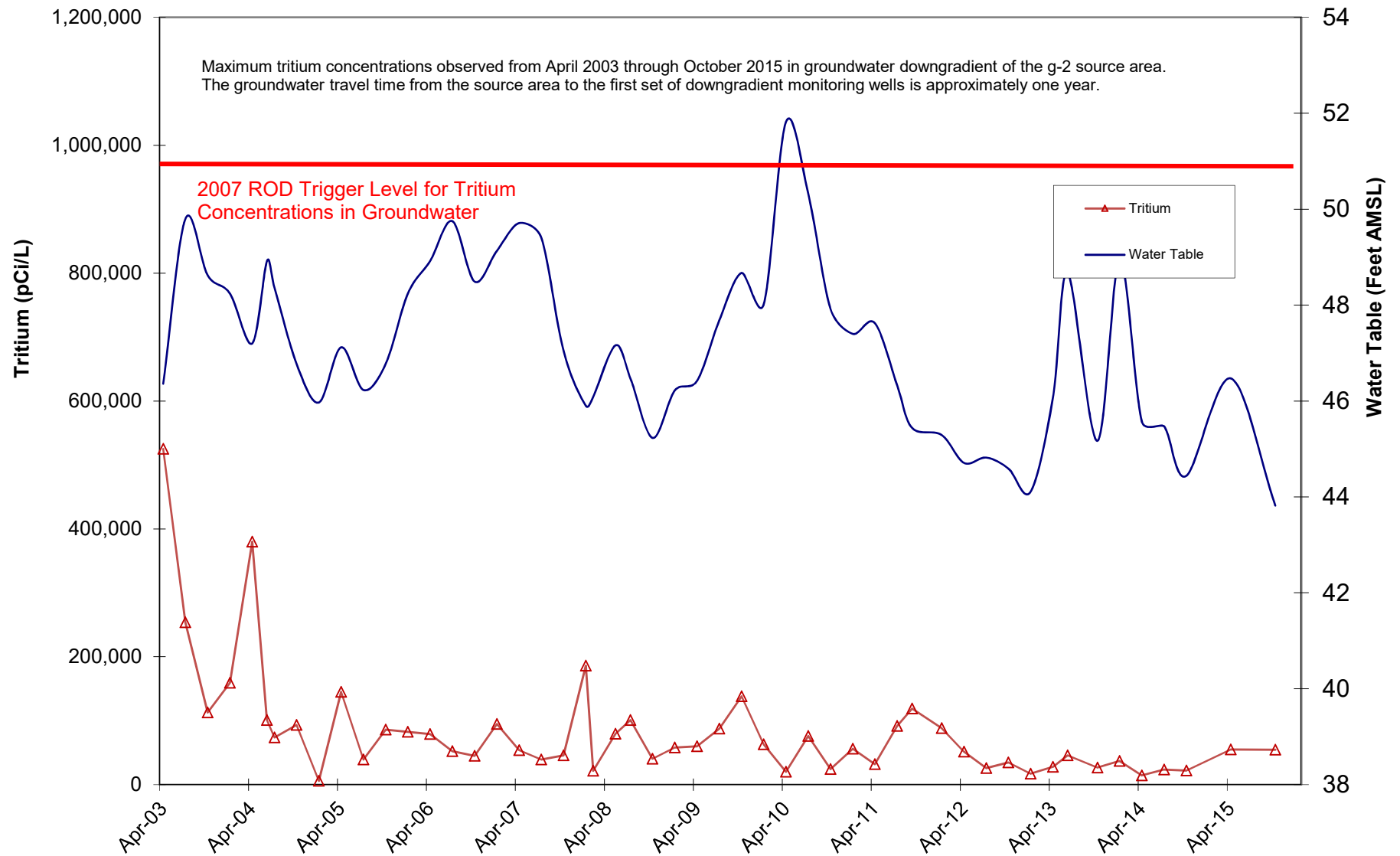
Figure 3.8-3 Facility Monitoring Program AOC 16T g-2 Tritium Plume Comparison to ROD Trigger
