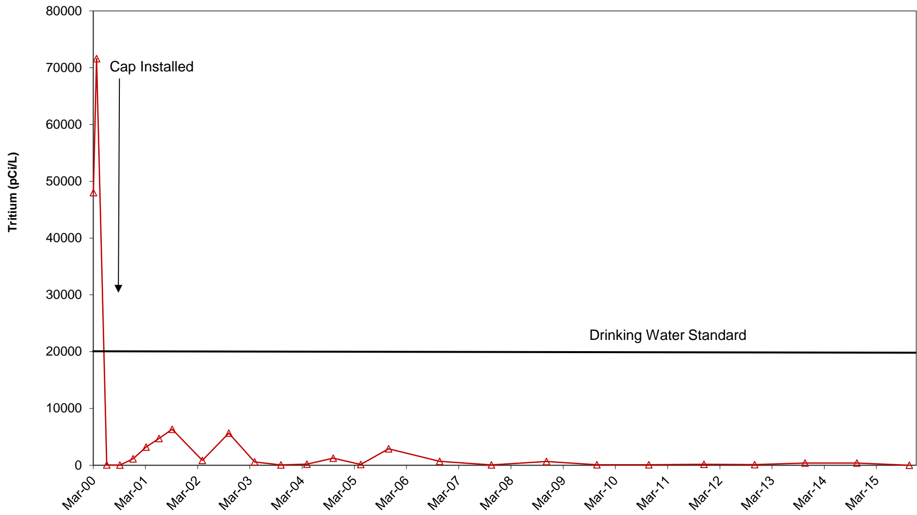
Figure 4.1-7 Facility Monitoring Program AGS Facility Area Maximum Tritium Concentrations Downgradient of Former U-Line Beam Stop Area
