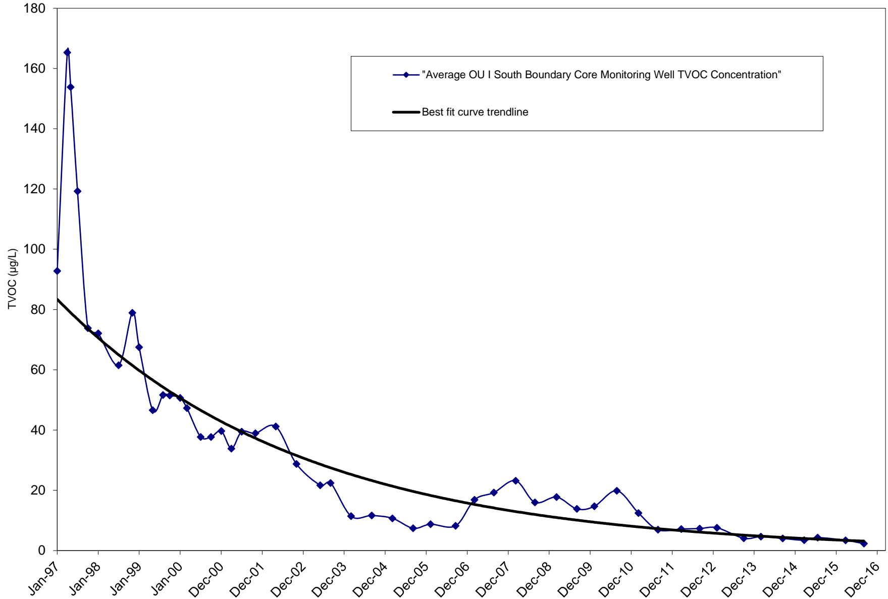
Figure 3.1-9 OU I South Boundary Groundwater Remediation System Average Core Monitoring Well TVOC Concentration
