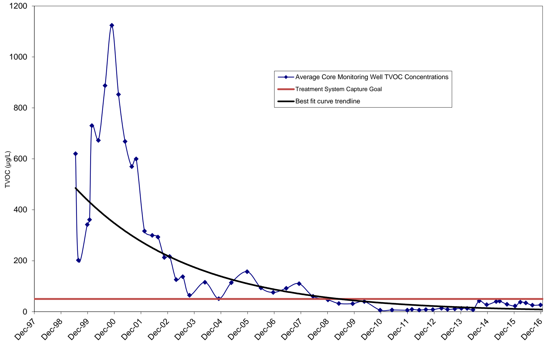
Figure 3.2.6-8 OU III Industrial Park Groundwater Remediation System Average Core Monitoring Well TVOC Concentration
