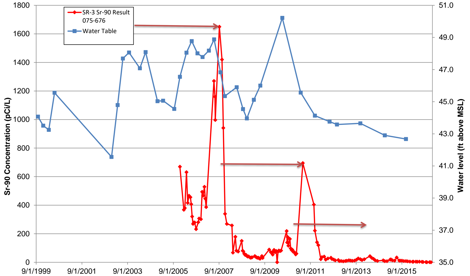
Figure 3.2.15-6 OU III BGRR/WCF Extraction Well SR-3 Sr-90 Concentration Comparison to Water Table Elevation
