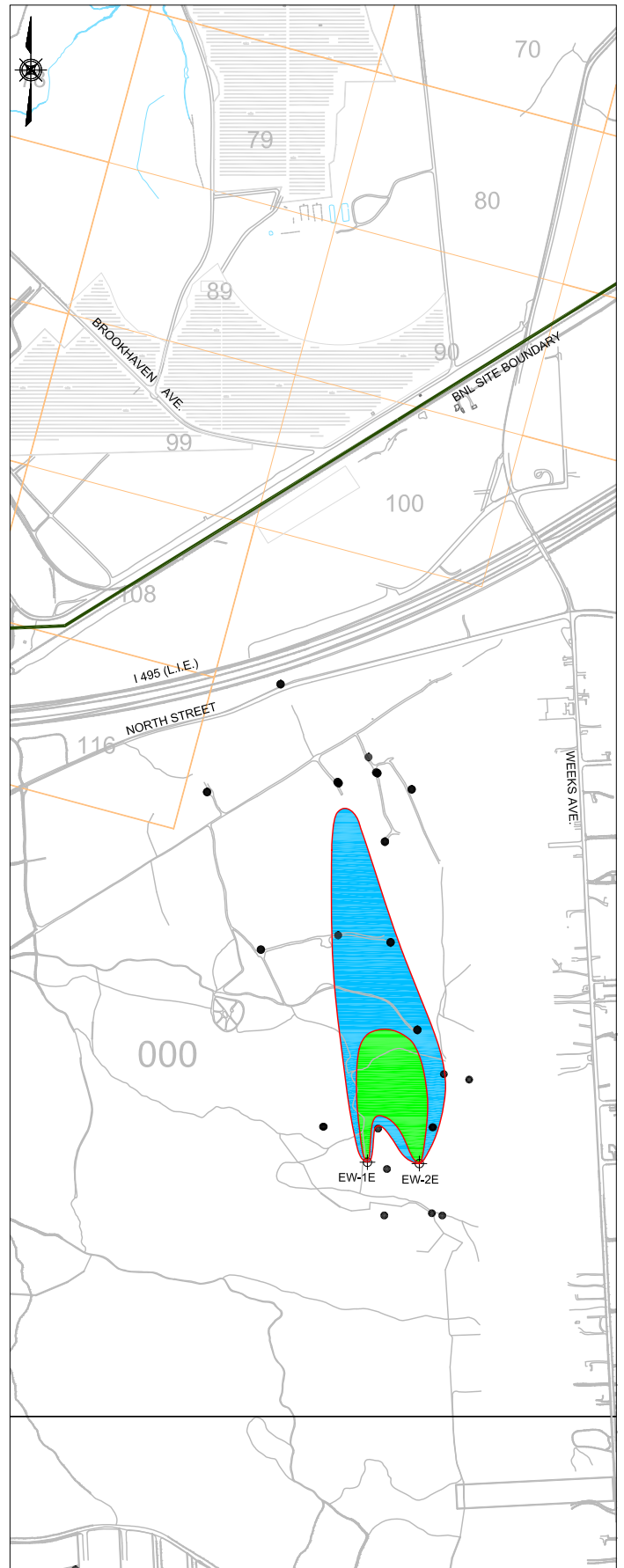
2016 EDB PLUME DISTRIBUTION
