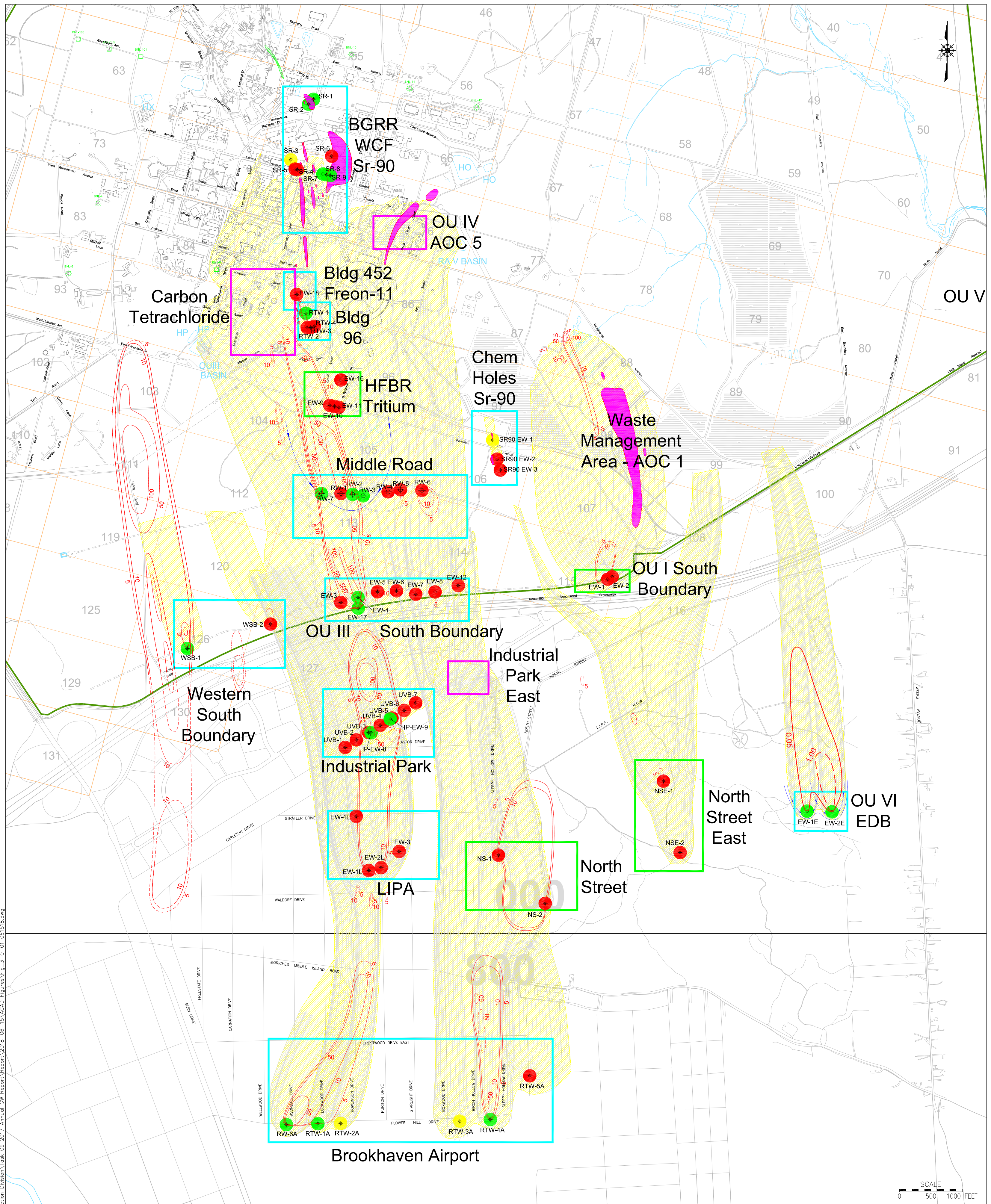
06/15/18 FIGURE: 3.0-1 GROUNDWATER REMEDIATION SYSTEMS
