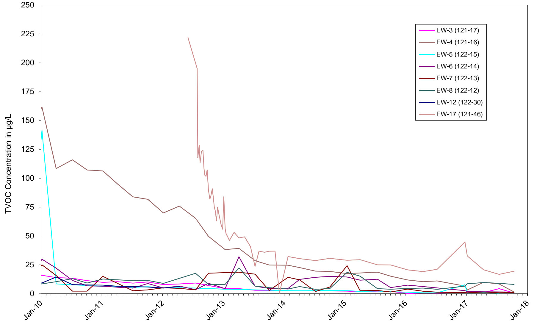
Figure 3.2.4-4 OU III South Boundary Groundwater Remediation System Total Volatile Organic Compounds in Extraction Wells 2010 through 2017
