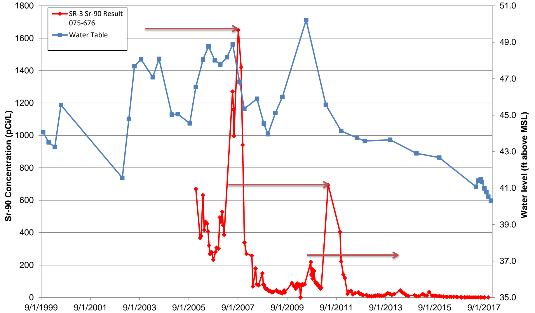
Figure 3.2.15-3 OU III BGRR/WCF Extraction Well SR-3 Sr-90 Concentration Comparison to Water Table Elevation
