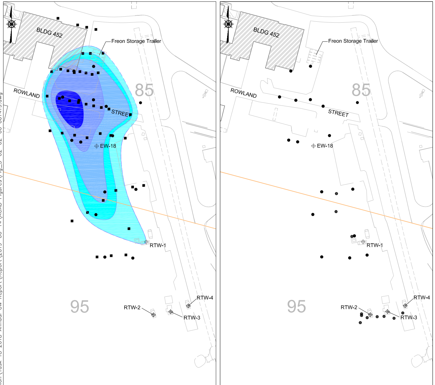
2011 FREON-11 PLUME
