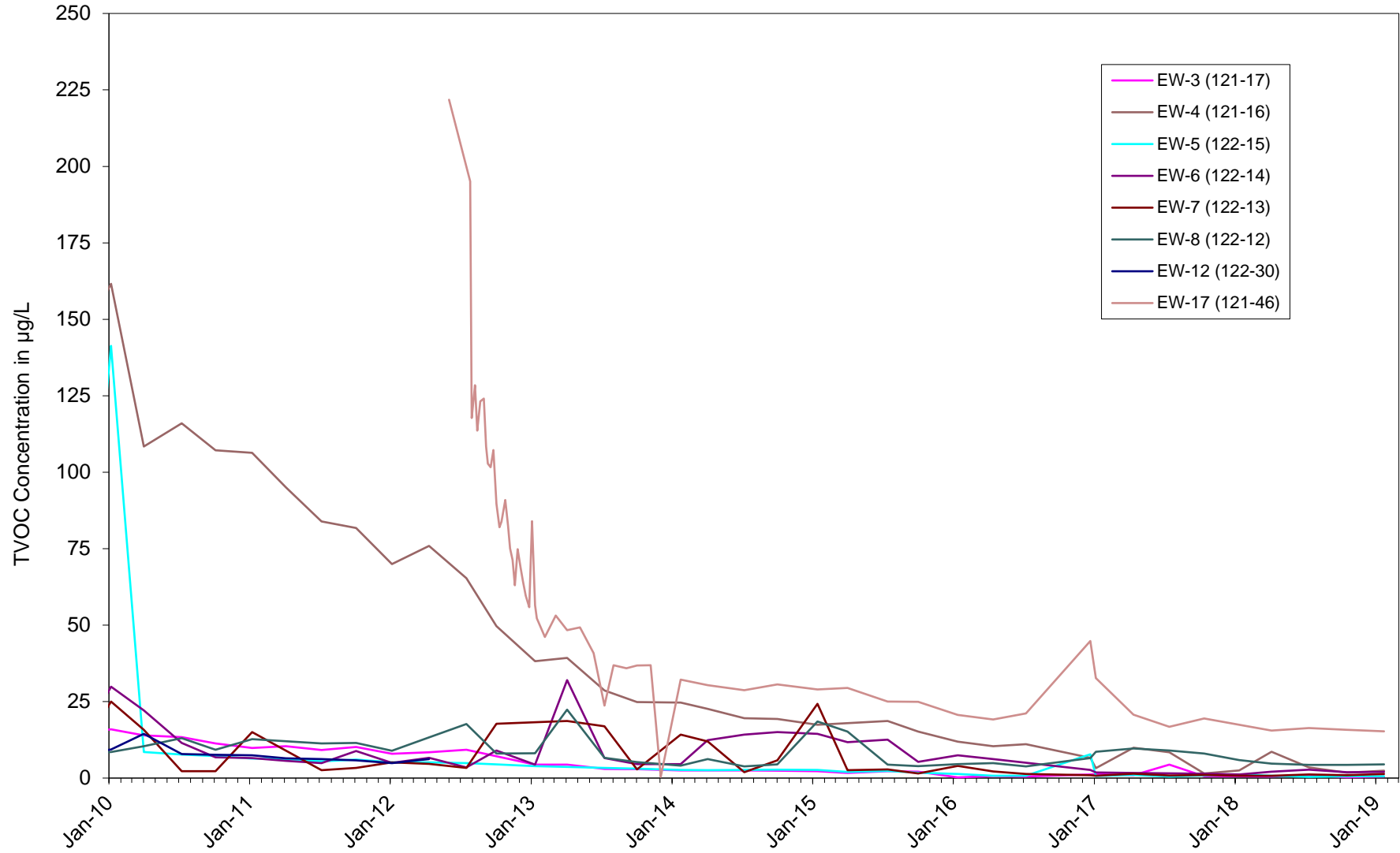
Figure 3.2.4-4 OU III South Boundary Groundwater Remediation System Total Volatile Organic Compounds in Extraction Wells 2010 through 2018
