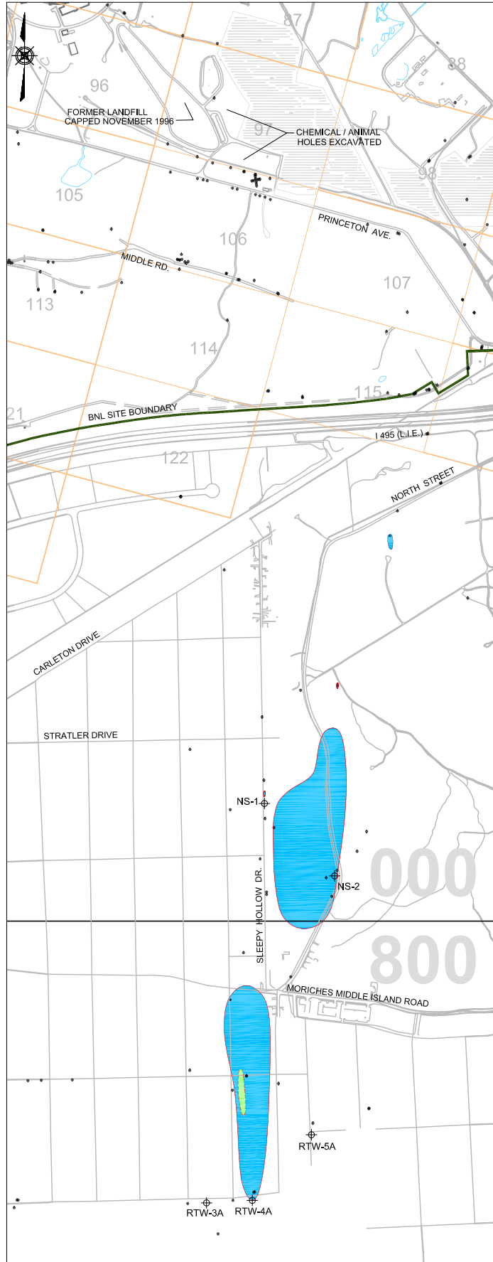
2018 TVOC PLUME DISTRIBUTION
