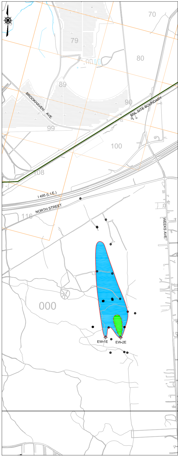
2018 EDB PLUME DISTRIBUTION
