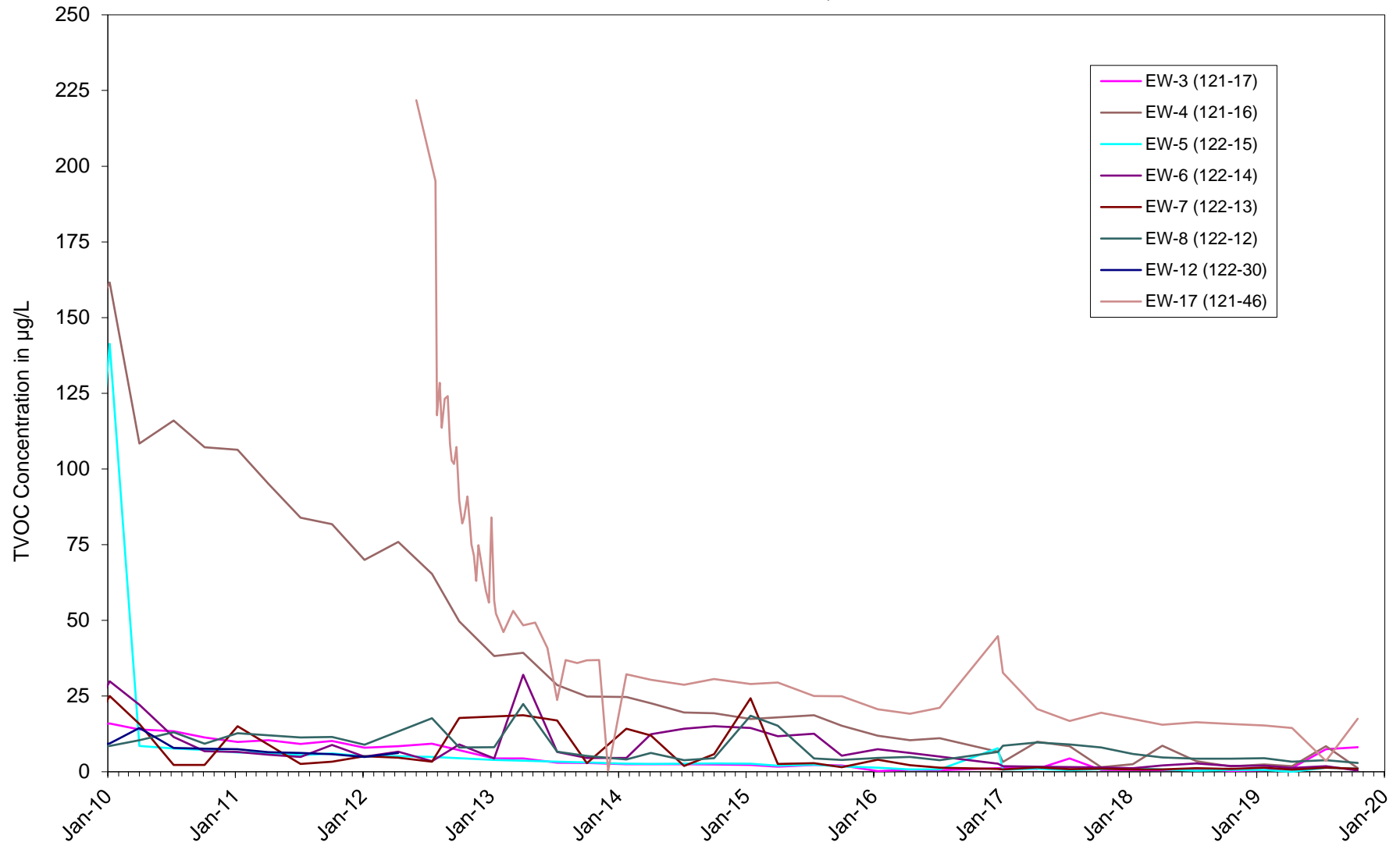
Figure 3.2.4-4 OU III South Boundary Groundwater Remediation System Total Volatile Organic Compounds in Extraction Wells 2010 through 2019
