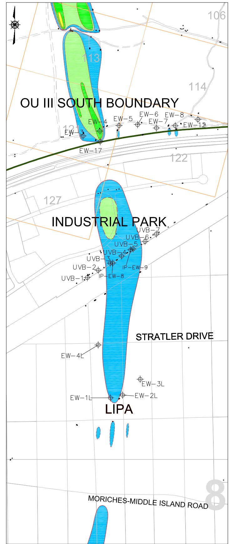
2019 TVOC PLUME DISTRIBUTION
