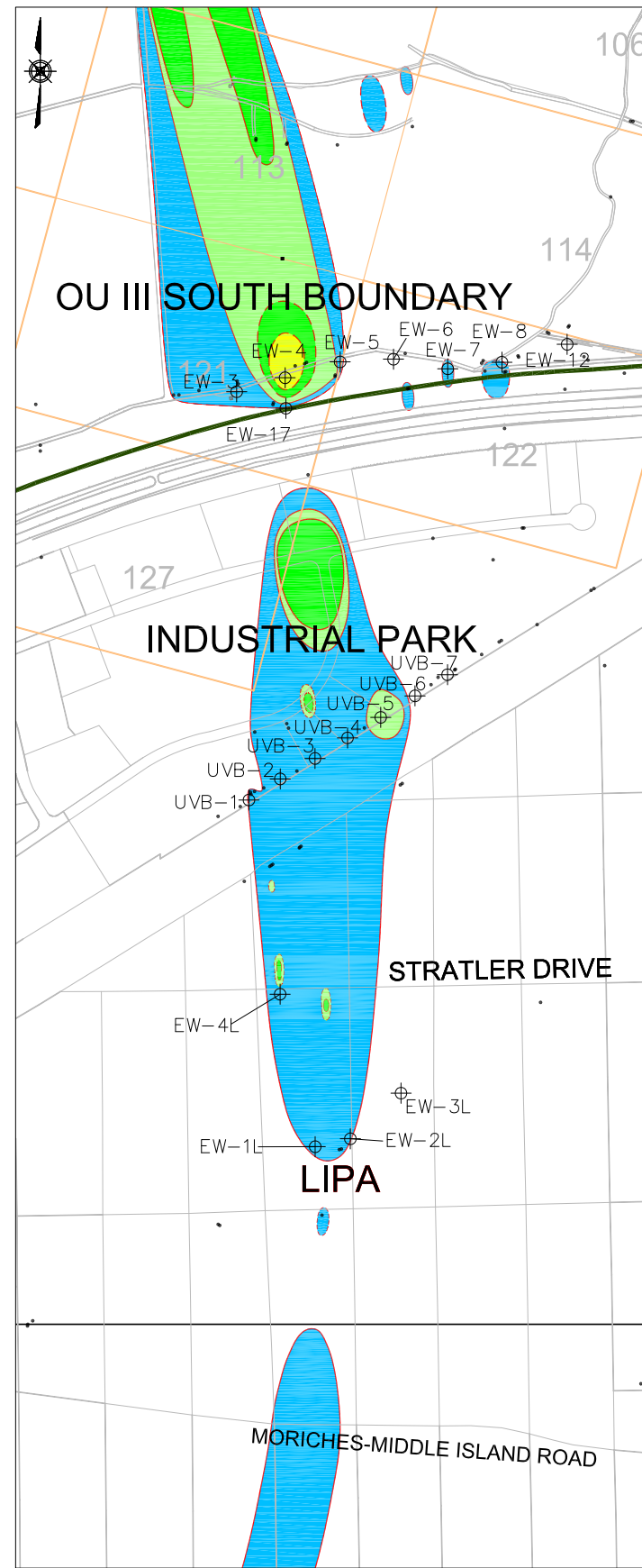
2013 TVOC PLUME DISTRIBUTION
