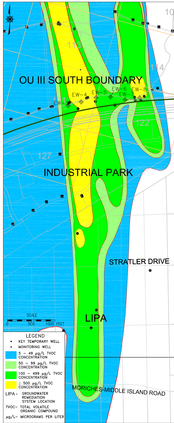
1997 TVOC PLUME DISTRIBUTION
