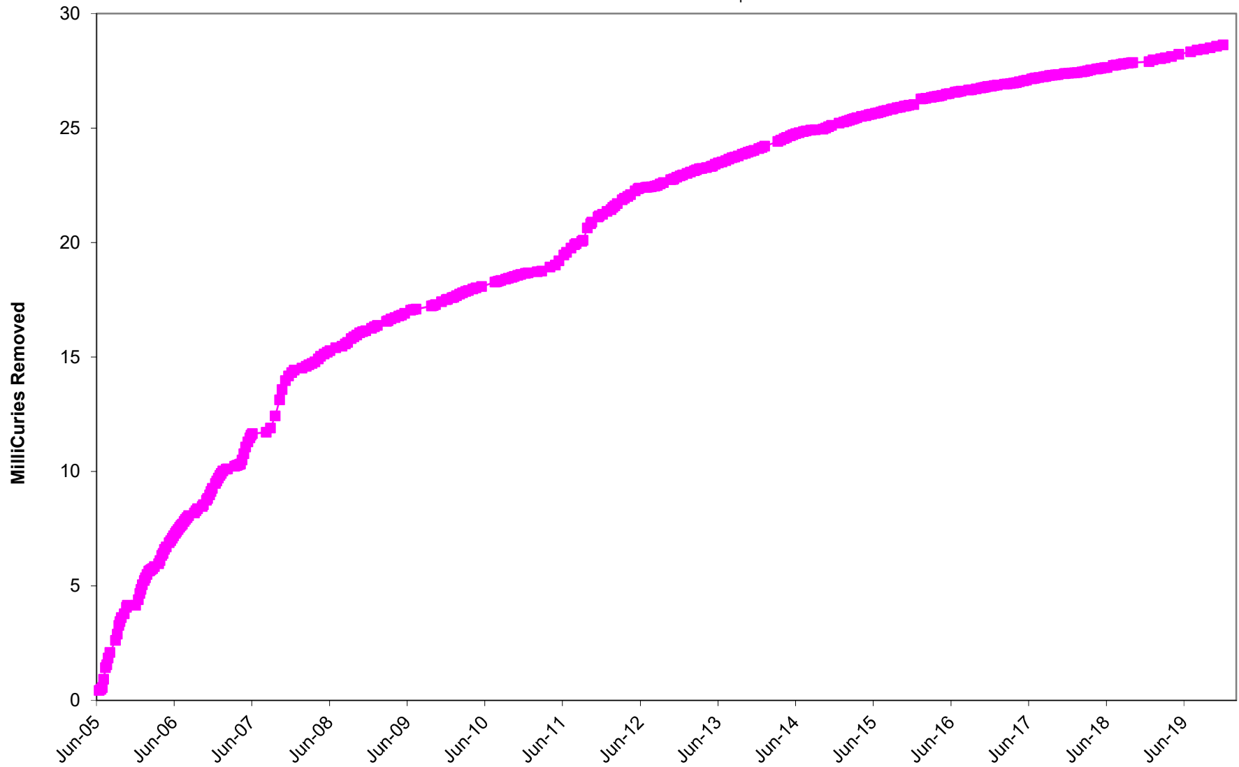
Figure 3.2.14-7 OU III BGRR/WCF Sr-90 Cumulative MilliCuries Removed
