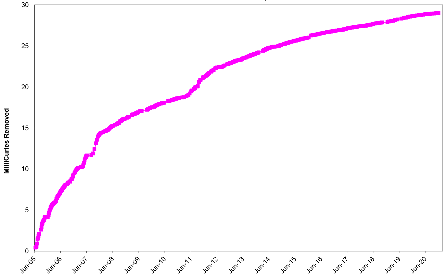
Figure 3.2.11-7 OU III BGRR/WCF Sr-90 Cumulative MilliCuries Removed
