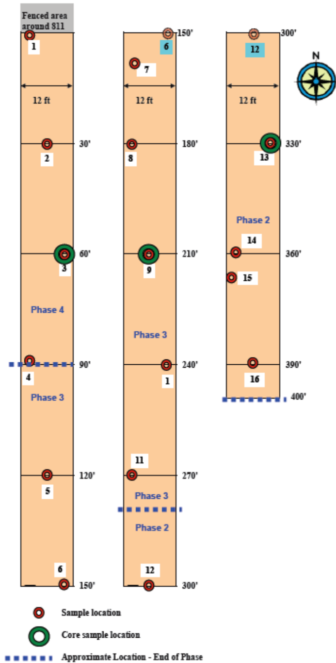
Figure 3-2 – Waste Transfer Line Survey Unit 1 soil and core sample locations
