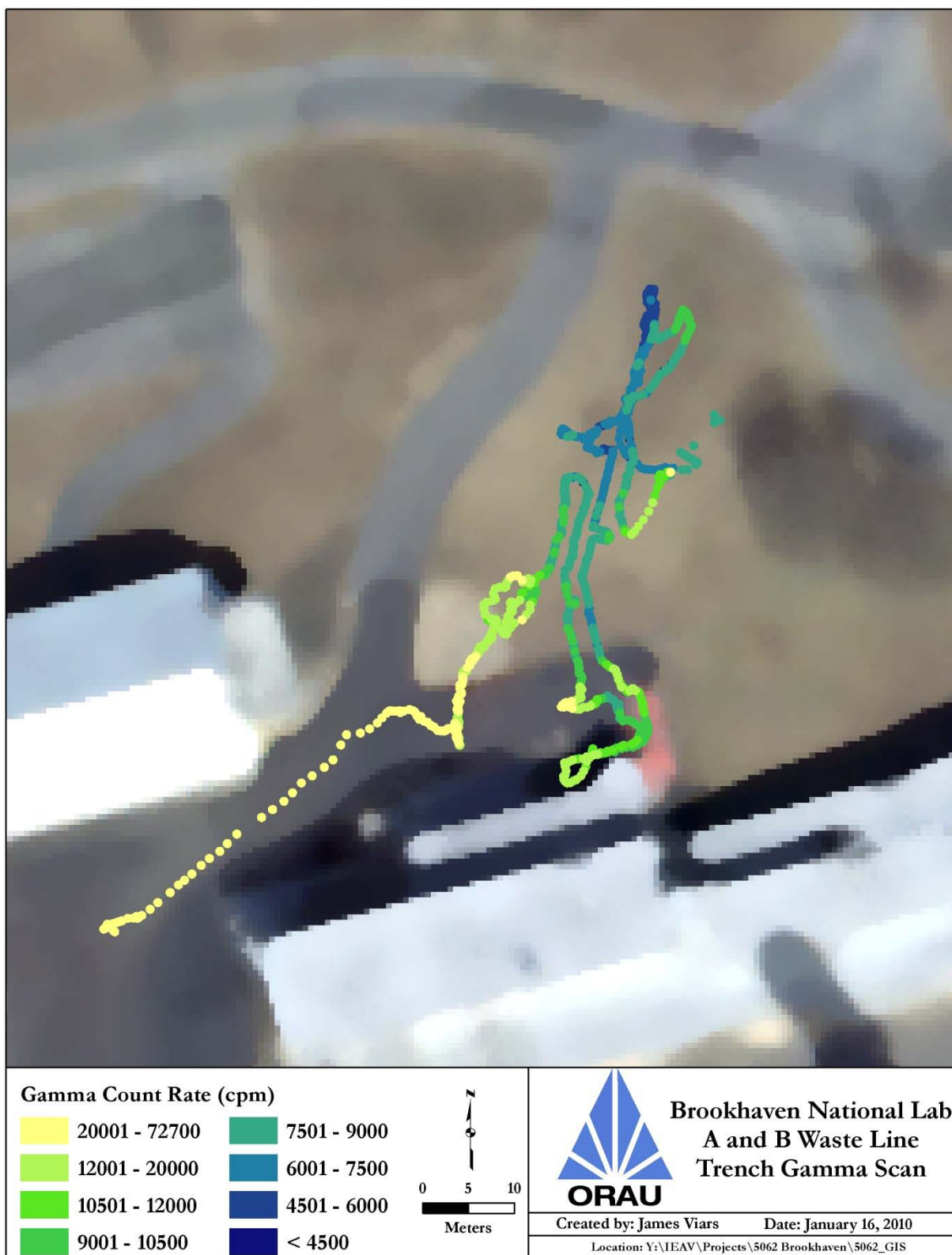
Figure A - 3: A and B Radioactive Waste Line Trench Gamma Activity Scan Pattern
