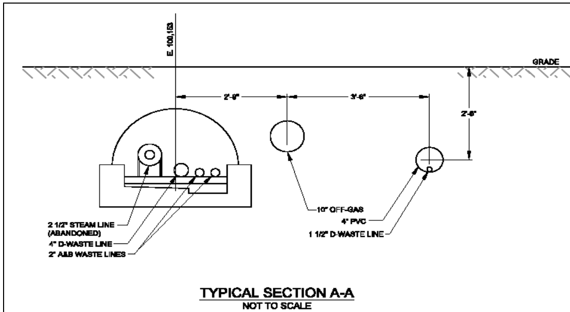
Figure 1-4 Typical Cross-Section of the Waste Transfer Lines
