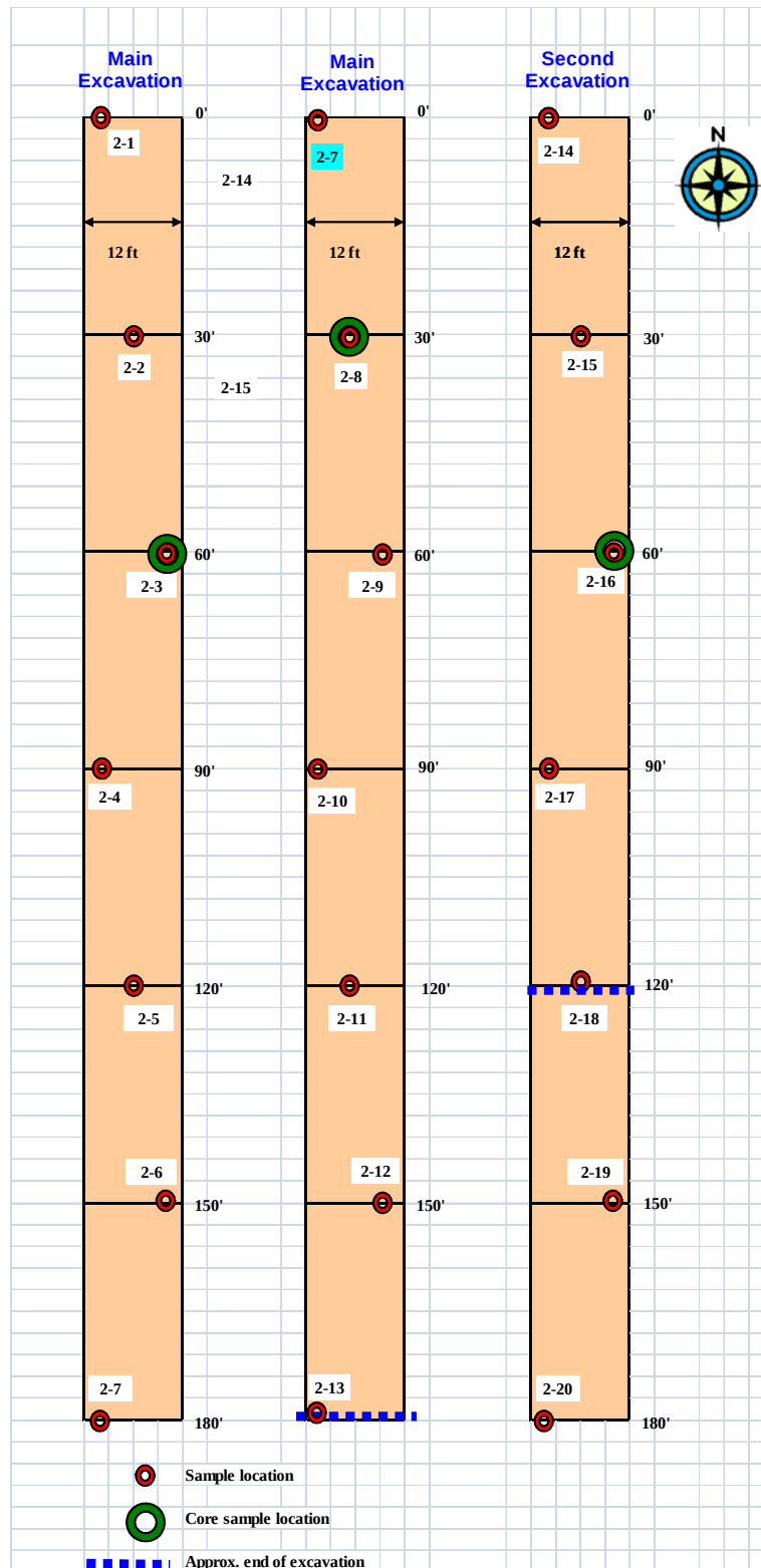
Figure 3-3 – Waste Transfer Line Survey Unit 2 soil and core sample locations
