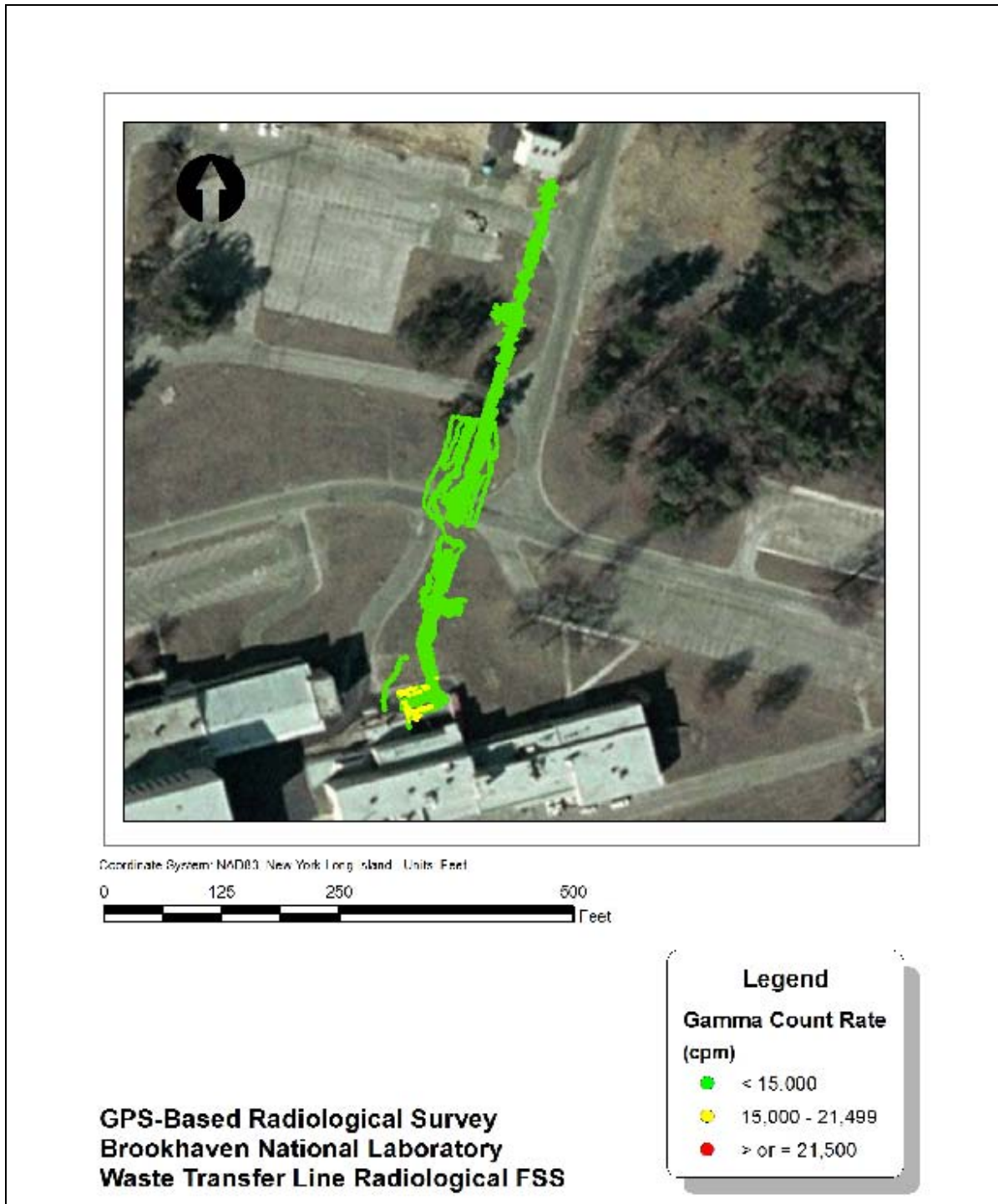
Figure 3-4 – Waste Transfer Lines post-remediation Radiological Walkover Survey results
