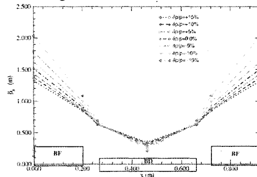
Fig. 1: Betatron functions in one gantry cell
