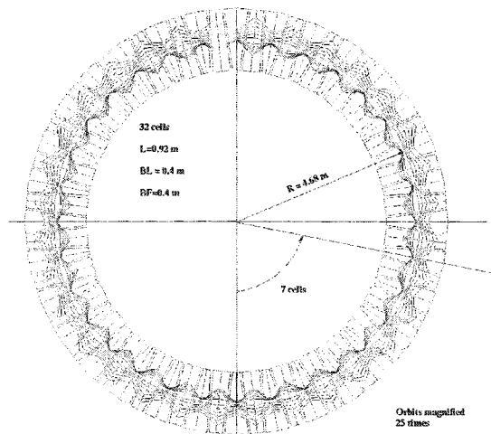
Fig. 3: Non-scaling FFAG ring to be used for the gantry design. Orbit offsets are magnified 25 times.
