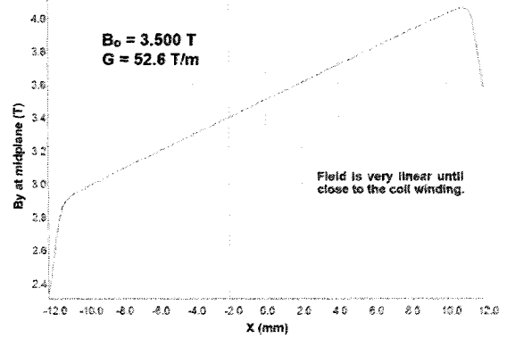
Fig. 9. Magnetic field along the transverse axis.
