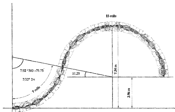
Fig. 4: A gantry made of 7 and 15 cells of the ring presented in previous figure. Orbit offsets are magnified 25 times. Tracking is performed with the PTC program.
