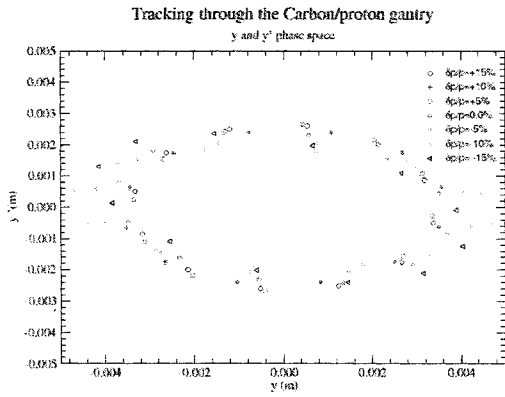
Fig. 7. Tracking results in the y, y' phase space.
