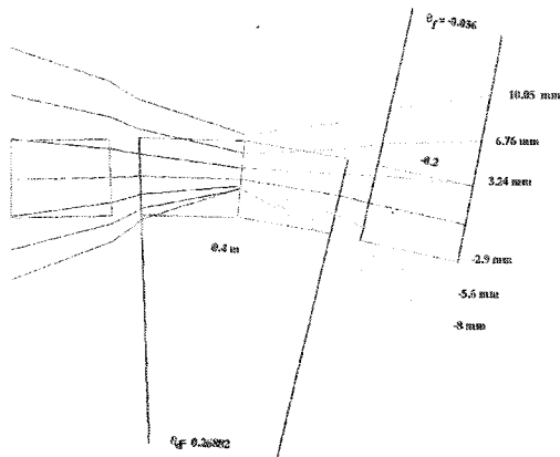
Fig. 2: The basic cell of the gantry made of non-scaling FFAG combined function magnets.
