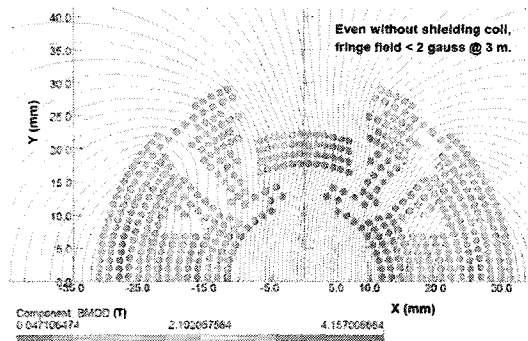
Fig. 8. Preliminary superconducting combined function magnet design.
