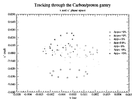
Figure 5: Tracking results in the x and x' phase space.
