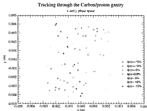
Figure 6: Tracking results in the x - y plane.
