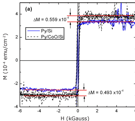
Room temperature hysteresis measurements for same thickness of Py deposited on Si (blue) and CoO/Si (black dashed). Red lines indicate the magnetization value at the positive and negative saturation for Py/Si and Py/CoO/Si, respectively.
