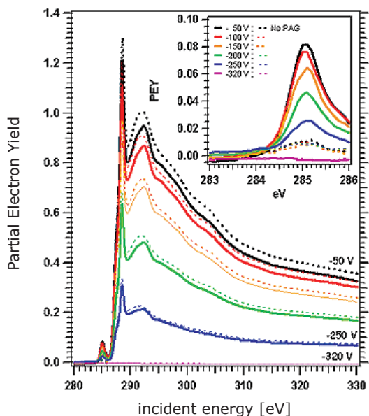
Figure 1. NEXAFS spectra of the pure photoresist (dotted lines) and resist containing 6.7 % by mass TPS-PFOS photoacid generator (solid lines) as a function of entrance-grid bias from -50 V to -250 V. At -320 V, no signal is detected. The inset highlights the \pi_{C=C}^* region which allows direct quantification of the triphenyl groups of the photoacid generator.
