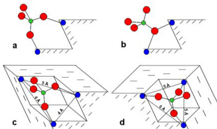
Figure 2. Schematic illustrations showing possible surface complexes for As(V) adsorption at step and kink sites on the calcite (10\bar{1}4) surface: (a) bidentate corner-sharing, (b) monodentate (bridging) corner-sharing, (c) tridentate corner-sharing at kink site in “-” step, (d) tridentate corner-sharing at kink site within “+” step.
