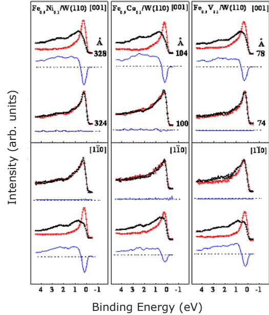
Figure 2. Typical result for magnetic reorientation transition as monitored with spin-resolved photoemission spectra of (a : \text{Fe}_{1-x}\text{Ni}_x ), (b : \text{Fe}_{1-x}\text{Co}_x ), and (c : \text{Fe}_{1-x}\text{V}_x ) at x = 0.1 concentration. The spectra were measured at 40 eV in normal emission. Each filled up-triangles and empty down-triangles represent majority- and minority- spin components, respectively. Below each spin resolved photoemission spectra, asymmetry values (I_{spin\ up} - I_{spin\ down}) / (I_{spin\ up} + I_{spin\ down}) also are displayed to show a clear change for spin reorientation for three alloy films. I_{spin\ up} and I_{spin\ down} indicate the intensity of majority spin and minority spin, respectively.
