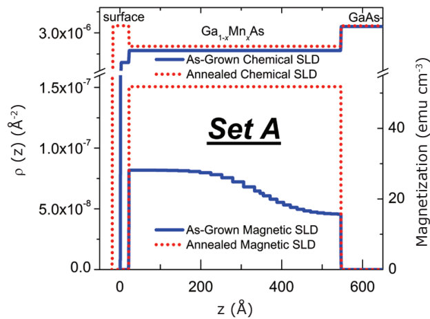
Figure 1. Scattering length density models of the as-grown (blue) and annealed (red) films, as deduced from polarized neutron reflectometry. The chemical depth profiles are shown above the break in the vertical axis, the magnetic depth profiles are shown below.
