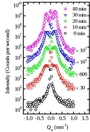
Figure 2. Time-resolved GISAXS measurements indicate the increase of the lateral correlations on a sapphire surface during ion exposure. The ion exposure was paused during the scans. The curves are shifted for clarity.
