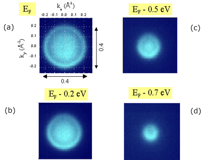
Figure 1. ARPES photocurrent intensity map of states within 1.5 eV of E_F , h\nu = 69 eV, and the sample temperature was 177 K. The sample was annealed to 300 °C in UHV for 30 minutes. The false color intensity reflects the photocurrent, with lighter intensity indicating higher current. The momentum direction is along \Gamma\Sigma M , in the surface plane.
