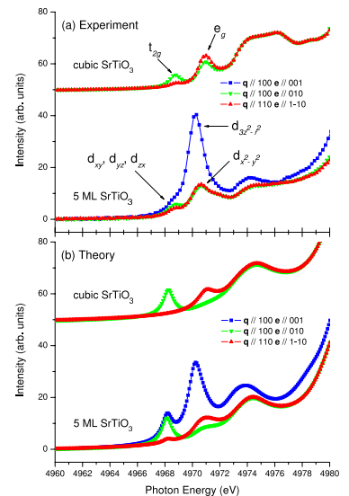
Figure 2: (a) Ti K spectra for cubic SrTiO 3 and a 5 monolayer (ML) SrTiO 3 thin film grown coherently on Si(001). (b) Theoretical spectra using the structures from Figure 1 (see text).
