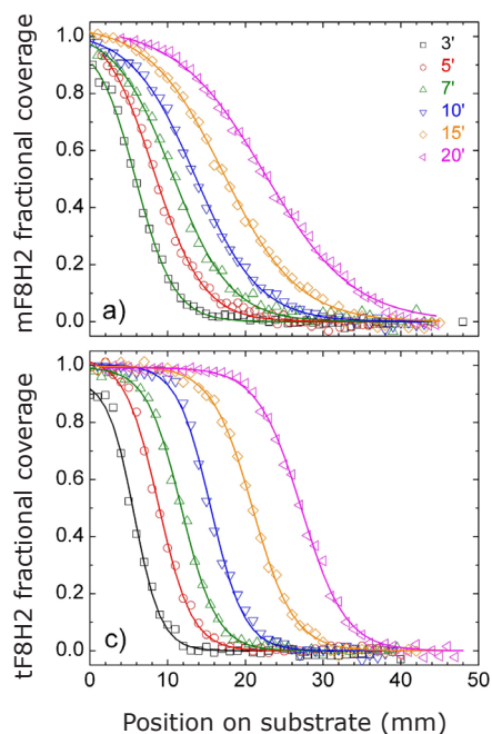
Figure 2. Time development of mF8H2 and tF8H2 surface energy gradients. The figures indicate mF8H2 and tF8H2 fractional coverage, respectively, as a function of substrate position for a succession of times. Fractional coverage refers to the OS concentration relative that for the fully ordered layer. Lines represent best fits to a hyperbolic tangent function as discussed in the original publication.
