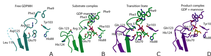
Figure 2. Snapshots of the catalytic cycle of GDPMH. (A) Crystallographic structure of the free enzyme. In this structure, loop L6 (dotted line) is disordered at the beginning of the cycle (pdb id 2GT2). (B) X-ray structure of the substrate complex. In this structure, although loop L6 becomes ordered, it remains in an "open" conformation (PDB id 1GT4). (C) Model of the GDPMH-transition state complex. This model was obtained by combining the coordinates of the enzyme in the product structure with the position of the GDP-mannose in the substrate structure (PDB id 2GT4) distorting the mannose to a half chair and elongating the mannosyl C1-GDP bond. In this model, loop L6 is in the "closed" conformation, bringing residues Gln123 and His 124 into their active positions. This conformational change is probably triggered by the positive charge developing on C1 of the mannose in the partially dissociative transition state acting on the negative charges in loop L6 (Asp-121, Glu-122, and Asp-125). (D) Product complex. This structure corresponds to the stage in the catalytic cycle before the release of products (PDB id 1RYA).
