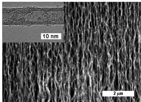
Figure 2. Scanning electron microscopy (SEM) image of a vertically aligned multiwall carbon nanotube forest. Inset: transmission electron microscopy image of a single multiwall carbon nanotube. Small angle x-ray scattering (SAXS) provides quantitative characterization of the alignment, where only qualitative assessments of orientation can be made with SEM. SAXS measurements yield a "locally averaged" measurement of the CNT diameter, where TEM requires imaging of individual nanotubes.
