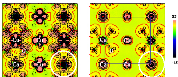
The bonding-electron distribution of CCTO containing Cu, Ca, and O atoms. (left) Experimental observation extracted from structure factor measurements using combined electron and x-ray diffraction data. (right) DFT calculation based on the ideal crystal structure.
