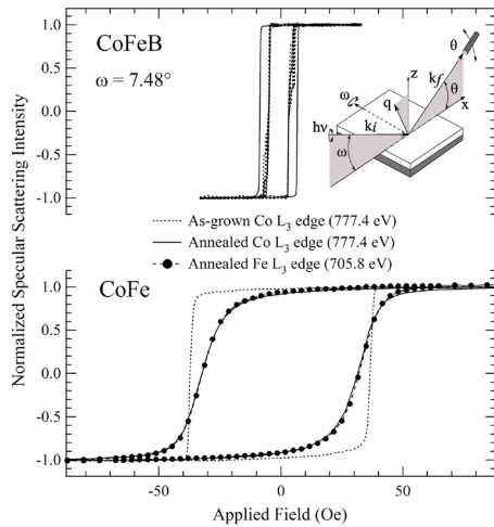
Figure 1. Specular scattering intensity for circular polarized x-rays at energies resonant with the Co L3-edge as a function of applied field for CoFeB (top panel) and CoFe (bottom panel) films as grown (dashed lines) and annealed (solid lines). Inset: configuration of the scattering setup.
