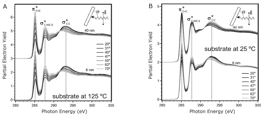
Figure 2 . (A) NEXAFS PEY spectra variation with incident angle for films deposited on hot substrates to 6 nm and 40 nm. (B) NEXAFS PEY spectra variation with incident angle for films deposited on room temperature substrates to 6 nm and 40 nm.
