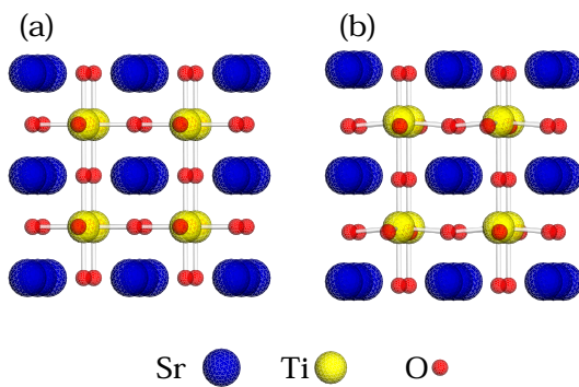
Figure 1: (a) Structure of cubic SrTiO 3 , (b) Structure of tetragonally distorted SrTiO 3 on Si(001) as calculated by DFT. The structure in (b) reveals both the AFD and FE distortions.
