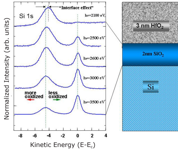
Figure 1. Si 1s spectra from 3nm \text{HfO}_2 / 2nm \text{SiO}_2 sample recorded with variable kinetic energy XPS illustrates depth profiling sensitivity and an interface effect near \text{HfO}_2
