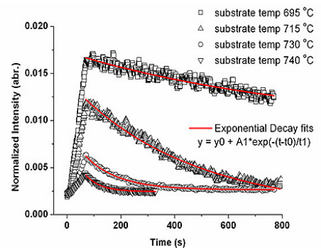
Figure 2. Ga fluorescence during (left) the absorption of Ga onto c-plane sapphire at different Ga cell temperatures and (right) during the desorption at different substrate temperatures.
