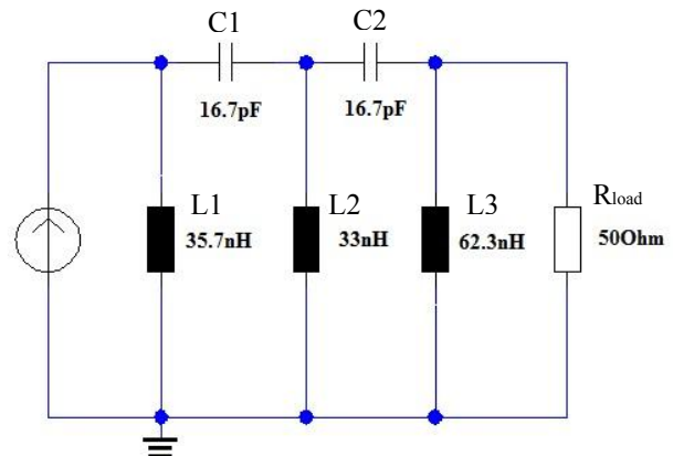
Figure 2: Simplified RLC circuit for high-pass filter.
