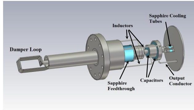
Figure 5: Engineering model of the filter.
