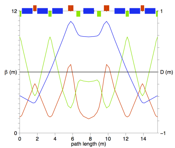
Figure 2: An isochronous cell with tune advance 0.95 and 0.525 in horizontal and vertical planes correspondingly.
