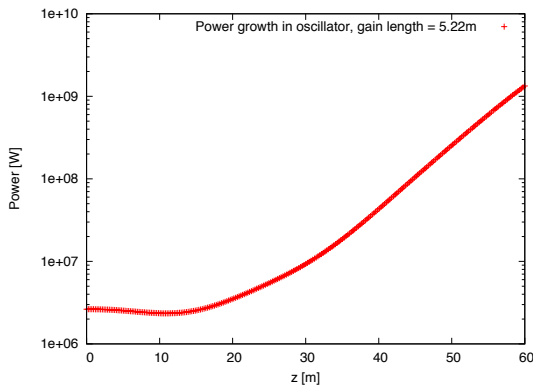
Figure 4: Power evolution inside the high gain FEL at the OFFELO saturation.
