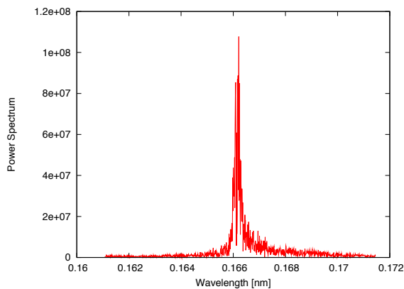
Figure 5: Radiation spectrum at pass #1 .
