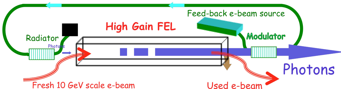
Figure 1. One of possible schemes for X-ray OFFELO. The central cube represents a high-gain X-ray FEL fed by a high-energy, 10 GeV scale, CW ERL. A low-energy electron beam energy-modulated by X-ray radiation exiting the FEL carries the imprinted modulation to its entrance. There the energy modulation is transferred into the density modulation and the beam radiates coherently in the radiator. This radiation is further amplified in the HGFEL, which completes the close loop of the oscillator.
