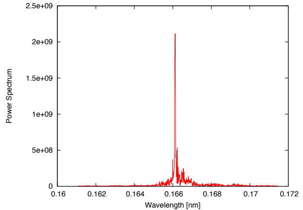
Figure 6: Radiation spectrum at pass #10 .
