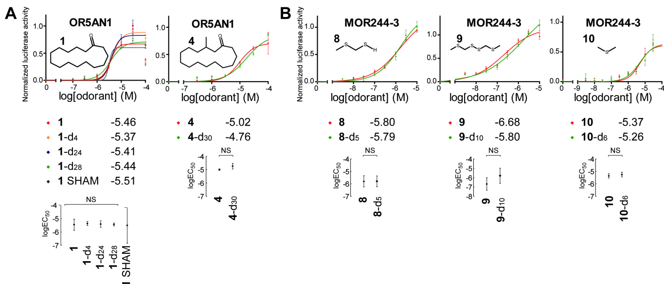
Fig. 3. Dose-response curves of (A) OR5AN1 to isotopomers of cyclopentadecanone (1) and muscone (4), and (B) MOR244-3 to isotopomers of MTMT (8), bis(methylthiomethyl) disulfide (9), and dimethyl sulfide (10). Best-fit logEC 50 values of the curves are shown alongside the graph legends (placed below the graphs). Scatter plots with 95% confidence interval logEC 50 values and indicating statistical significances between the logEC 50 values among isotopomers are also shown below the corresponding graphs. In B, 30 \mu M of copper was added upon odorant stimulation. "SHAM" indicates non-deuterated cyclopentadecanone subjected to the same chemical synthetic procedures as the deuterated samples without D 2 O addition. "NS", not significant. For all dose-response curve graphs, the chemical structures of the respective compounds are shown within the graphs and normalized responses are shown as mean \pm SEM ( N = 3 ).
