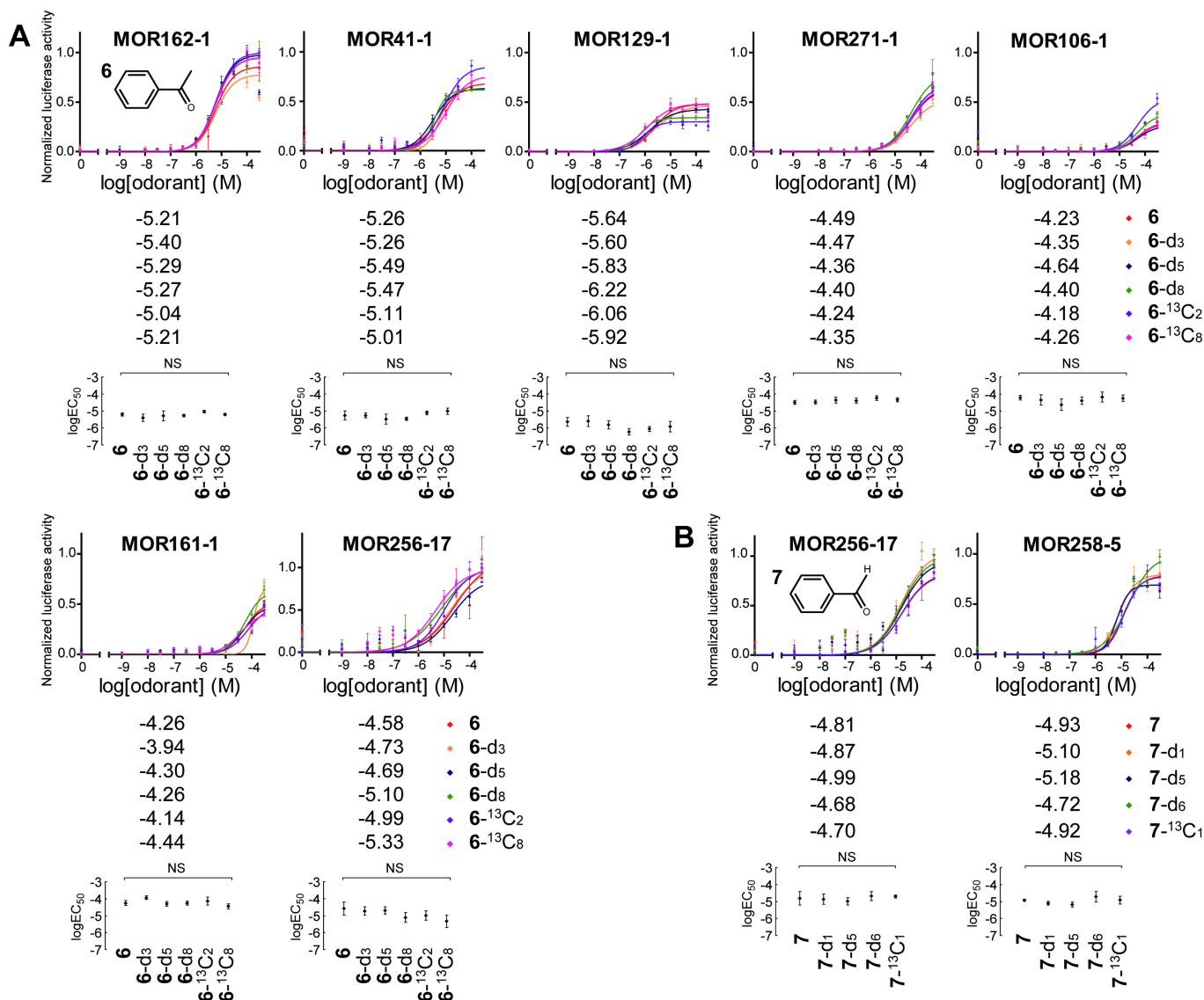
Fig. 4. Dose-response curves of various human and mouse receptors to isotopomers of (A) acetophenone (6) and (B) benzaldehyde (7). Best-fit logEC 50 values of the curves are shown alongside the graph legends (placed below the graphs). Scatter plots with 95% confidence interval logEC 50 values and indicating statistical significances between the logEC 50 values among isotopomers are also shown below the corresponding graphs. "NS", not significant.
