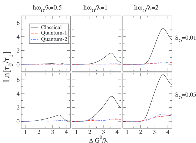
Fig. 5. The natural logarithms of the ratios of \tau_0/\tau_1 versus -\Delta G^0/\lambda (negative Gibbs free energy of reaction in the unit of reorganization energy) corresponding to the results in Figs. S1-3. The "Classical" refers to the classical limit of Ohmic bath, Eq. (18) of SI, with parameters for Fig. S1.1. The "Quantum-1" refers to the quantum regime of the Ohmic bath with parameters for Fig. S1.2. The "Quantum-2" refers to the case of classical Ohmic bath plus one quantum mode in the bath with parameters for Fig. S1.3. Each column represents different value of \hbar\omega_O/\lambda , where \omega_O is the angular frequency of the odorant oscillator and \lambda is the reorganization energy of the protein environments. The upper panels are for S_O = 0.01 and the lower panels are for S_O = 0.05 , where S_O is the Huang-Rhys factor for the odorant oscillator.
