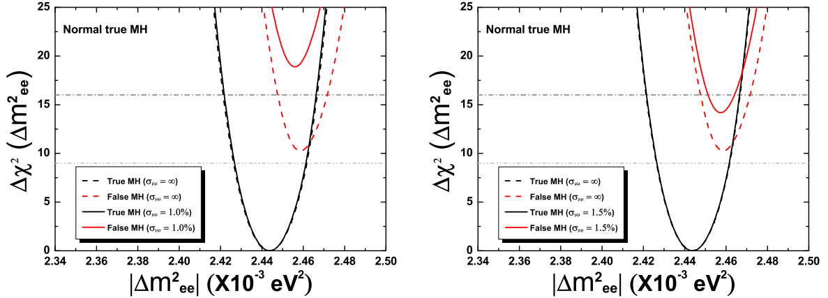
Figure 2-16: the reactor-only (dashed) and combined (solid) distributions of the \Delta\chi^2 function in Eq. (2.9) and Eq. (2.23), where a 1% (left panel) or 1.5% (right panel) relative error of \Delta m_{\mu\mu}^2 is assumed and the CP-violating phase ( \delta ) is assigned to be 90^\circ/270^\circ ( \cos\delta = 0 ) for illustration. The black and red lines are for the true (normal) and false (inverted) neutrino MH, respectively.
