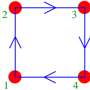
Fig. 3. Analogous to Stoke’s law, the flux through an elementary square of the lattice is found from the product of gauge matrices around that square. The dynamics is determined by adding the real part of the trace of this product over all elementary squares. This “action” is inserted into a “path integral.” The resulting construction is formally equivalent to a partition function for a system of “spins” existing in the group SU(3) .
