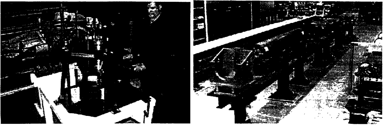
Figure 4: Left (a): Lamination stacking fixture. Right (b): Alignment table for assembling the cold mass of a complete snake or rotator. The first helical dipole is shown at the near end.
