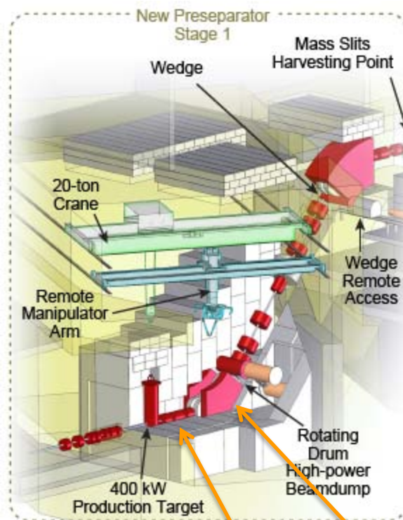
Pre-separator quads and dipole
