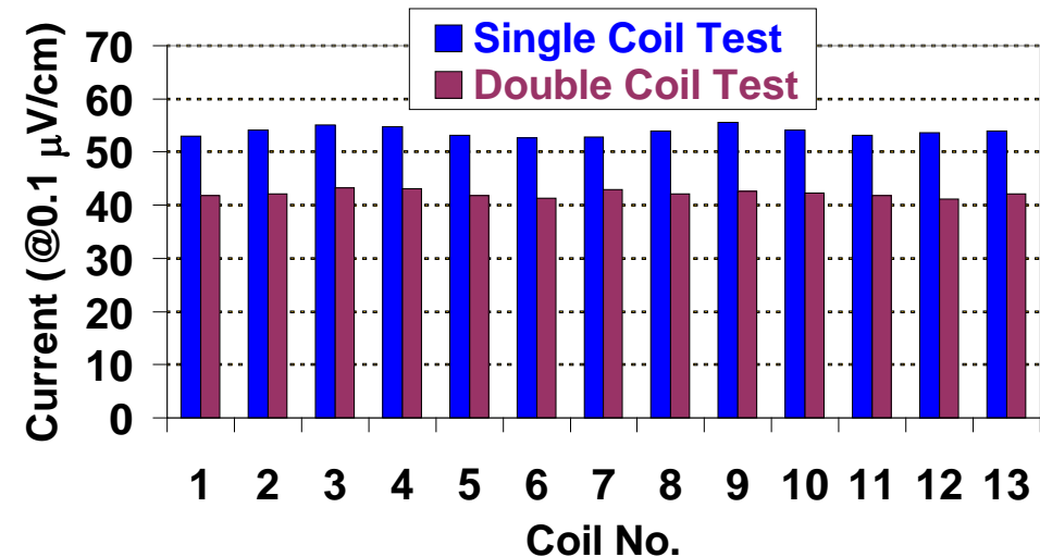
13 Coils made HTS tape in year #1
