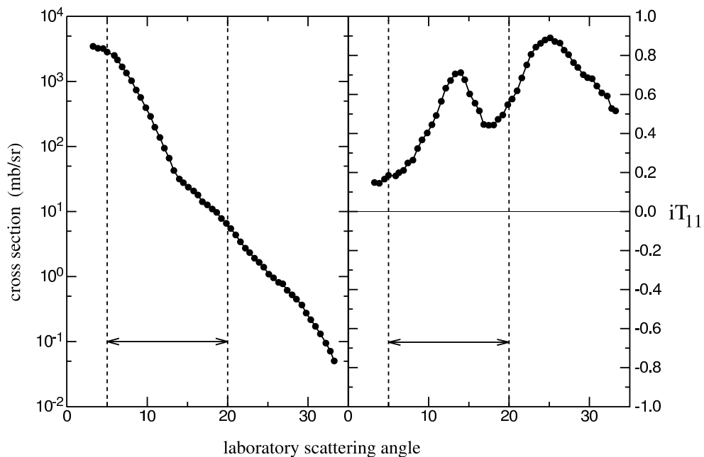
Figure 2: Deuteron elastic cross section and analyzing power at 270 MeV from carbon [25]. The dashed lines indicate the preferred acceptance limits for an EDM polarimeter.
