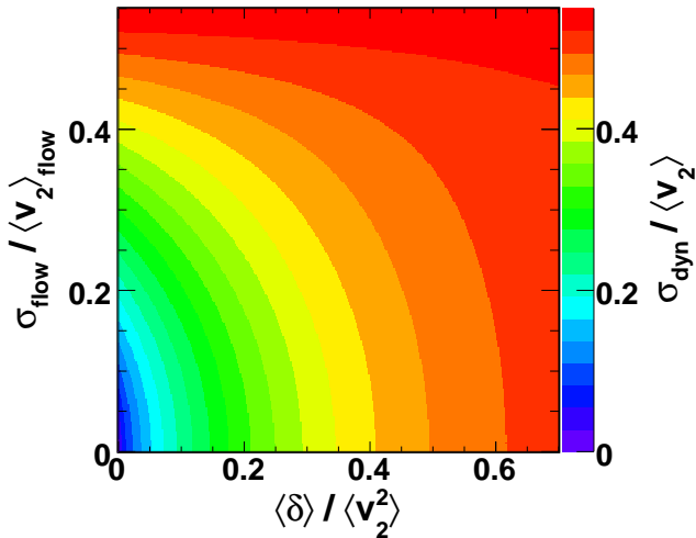
FIG. 7: Dynamic v_2 fluctuations ( \sigma_{\text{dyn}}/\langle v_2 \rangle ) as a function of elliptic flow fluctuations ( \sigma_{\text{flow}}/\langle v_2 \rangle_{\text{flow}} ) and the non-flow ratio ( \langle \delta \rangle / \langle v_2^2 \rangle ) for \sigma_n / \langle v_2 \rangle_{\text{flow}} = 0.6 . The observed values of dynamic v_2 fluctuations are roughly given by \sigma_{\text{dyn}}/\langle v_2 \rangle \approx 40\% [11].
