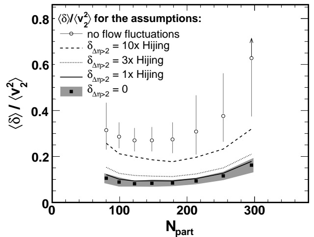
FIG. 5: The non-flow ratio ( \langle \delta \rangle / \langle v_2^2 \rangle ) in the PHOBOS Octagon detector acceptance as a function of number of participating nucleons ( N_{\text{part}} ) in Au+Au collisions at \sqrt{s_{NN}} = 200 GeV. The black squares show the results with the assumption that non-flow correlations are negligible at |\Delta\eta| > 2 . The shaded band shows the 90% confidence systematic errors. The lines show different assumptions about non-flow at |\Delta\eta| > 2 . The open circles with 90% C.L. systematic errors, show the upper limit on \langle \delta \rangle / \langle v_2^2 \rangle obtained by assuming that the measured dynamic fluctuations in v_2 are due to non-flow alone.
