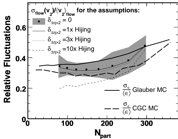
FIG. 6: Relative elliptic flow fluctuations ( \sigma_{\text{flow}}/\langle v_2 \rangle_{\text{flow}} ) as a function of number of participating nucleons ( N_{\text{part}} ) in Au+Au collisions at \sqrt{s_{\text{NN}}} = 200 GeV. The black circles show the results with the assumption that non-flow correlations are negligible at |\Delta\eta| > 2 . The shaded band shows the 90% confidence systematic errors. The thin lines show results for different assumptions on the magnitude of non-flow at |\Delta\eta| > 2 . The continuous and dashed thick lines show \sigma(\epsilon_{\text{part}})/\langle \epsilon_{\text{part}} \rangle values calculated in Glauber MC [11] and CGC [24] models, respectively.
